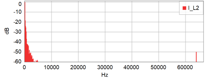
Fig. 15. Spectral analysis of L2 current signal
