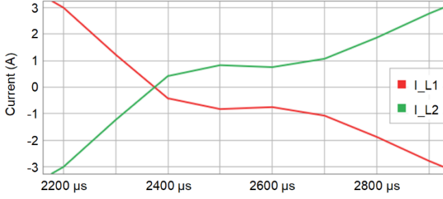
Fig. 6. 10 kps current zero crossing
