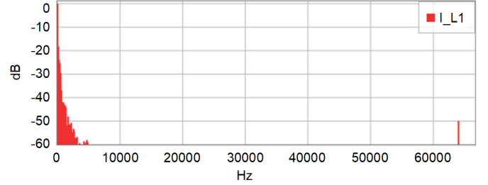
Fig. 14. Spectral analysis of L1 current signal
