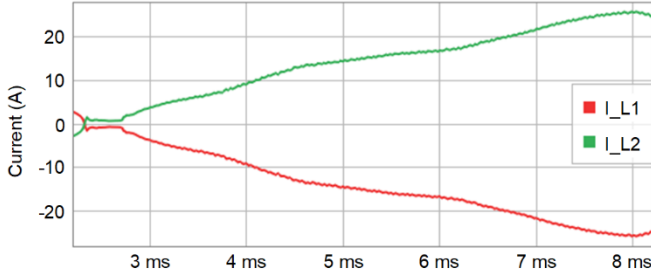
Fig. 8. 6 ms, 1 Msps current waveform
