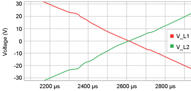
Fig. 7. Msps voltage zero crossing
