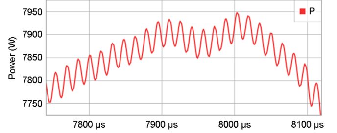
Fig. 13. Instantaneous power ripple
