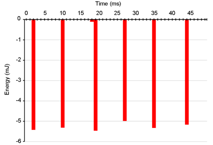
Fig. 18. Negative 1 ms energy packets
