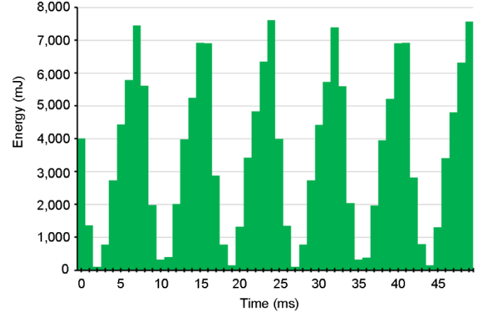
Fig. 17. Positive 1 ms energy packets
