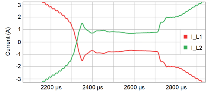
Fig. 5. 1 Msp/s current zero crossing
