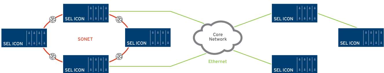
Mixed transport with linear spurs.
