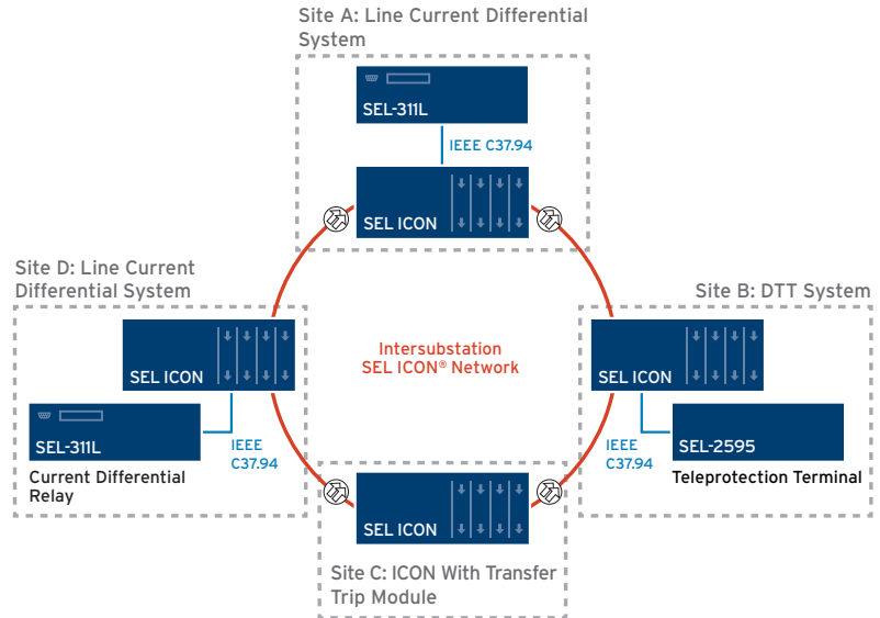
Example of teleprotection communication for protecting a transmission system.
