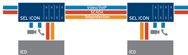
Example of segregating IEC 61850 traffic from other applications.
