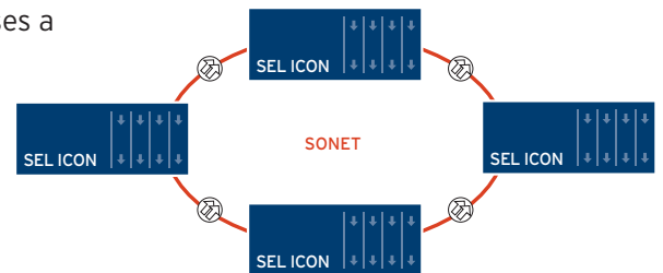
Single-ring topology.
