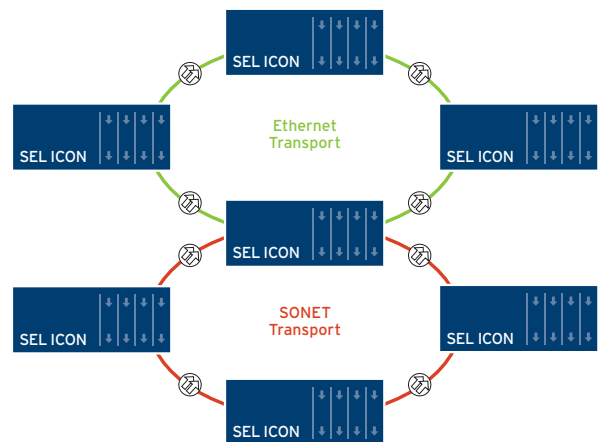
Mixed SONET and Ethernet transport.
