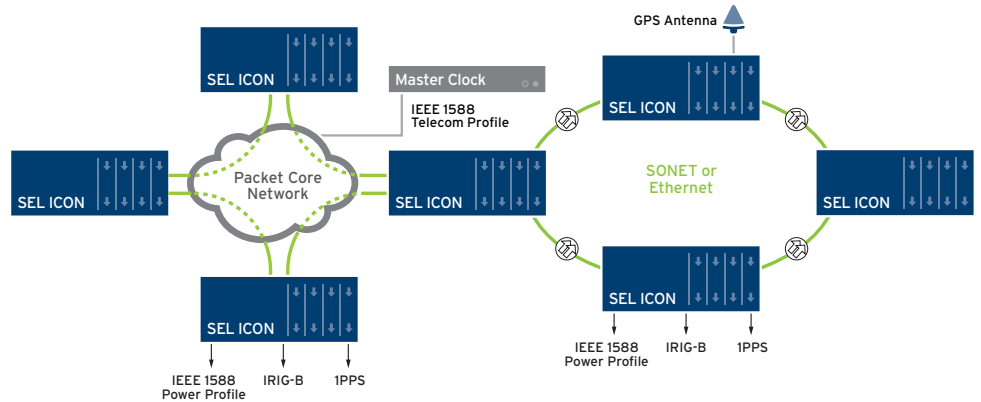
Example network time distribution application. ICON nodes are synchronized across the WAN and generate time references for substation device synchronization.
