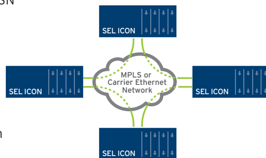
Single-ring core transport topology.
