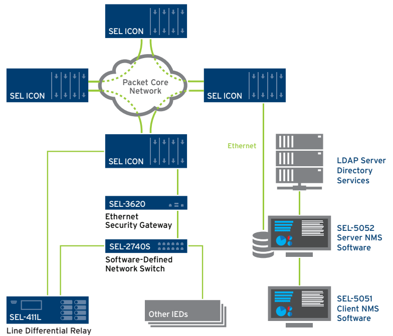
ICON network management.
