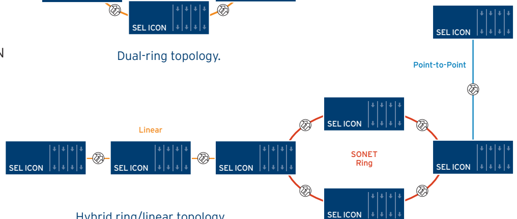
Hybrid ring/linear topology.
