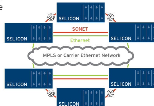
Single-ring mixed transport topology.
