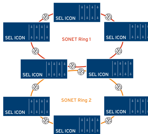
Dual-ring topology.
