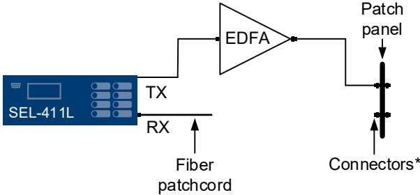
Figure 2 Application Example of a Booster Amplifier
