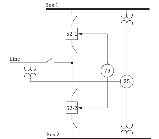
Figure 5 Two-Breaker Reclosing With Synchronism Check
