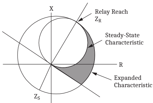
Figure 3 Mho Characteristic
