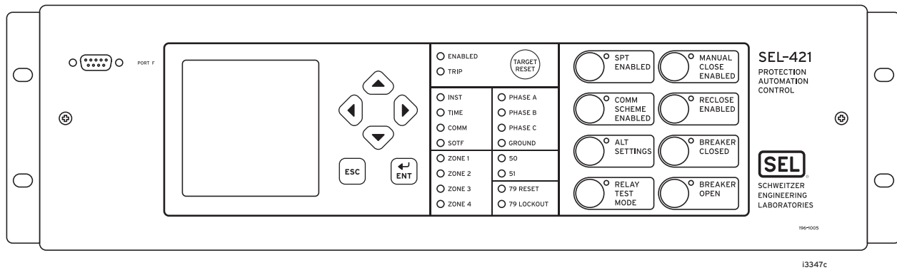
Figure 25 3U Front Panel, Rack-Mount Option With Standard HMI
