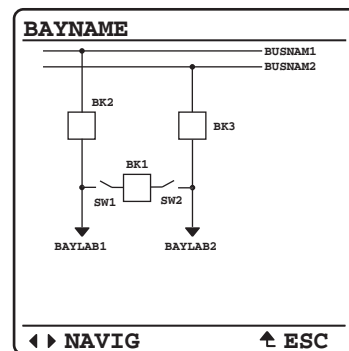
Figure 12 Breaker-and-a-Half
