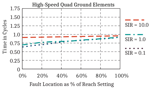
Figure 4 Quadrilateral Single-Phase-to-Ground Faults
