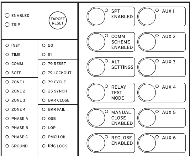
Figure 10 Factory-Default Status and Trip Target LEDs (12 Pushbutton, 24 Target LED Option)
