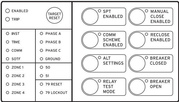
Figure 9 Factory-Default Status and Trip Target LEDs (8 Pushbutton, 16 Target LED Option)
