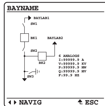
Figure 13 Ring Bus With Ground Switch
