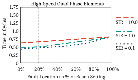
Figure 5 Quadrilateral Phase-to-Phase Faults
