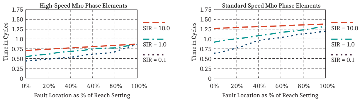
Figure 3 Mho Phase-to-Phase Faults
