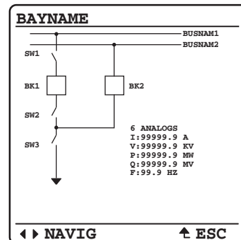
Figure 14 Double Bus/Double Breaker
