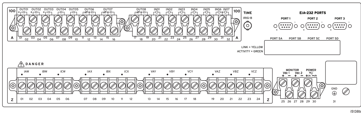
Figure 27 3U Rear Panel, Main Board With Terminal Block
