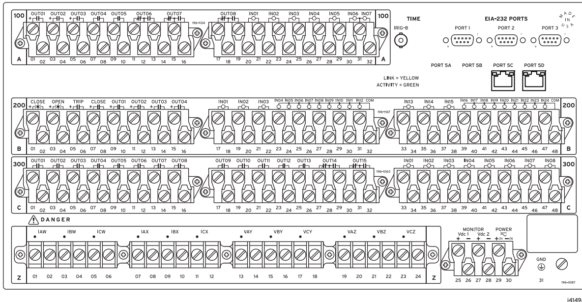
Figure 29 5U Rear Panel, Main Board With Terminal Block and Two (One INT3 and One INT2) I/O Boards
