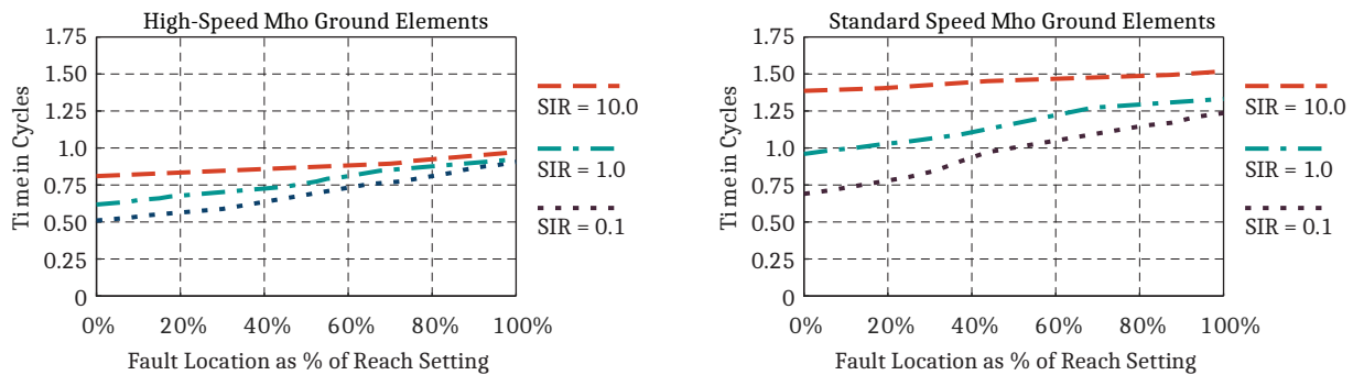
Figure 2 Mho Single-Phase-to-Ground Faults
