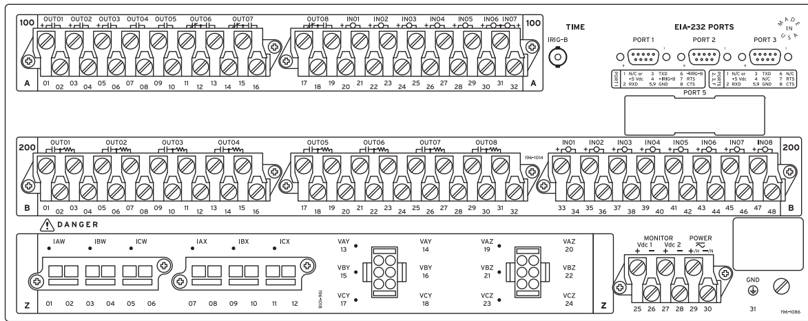
Figure 28 4U Rear Panel, Main Board, Connectorized® Option With One (INT5) I/O Board
