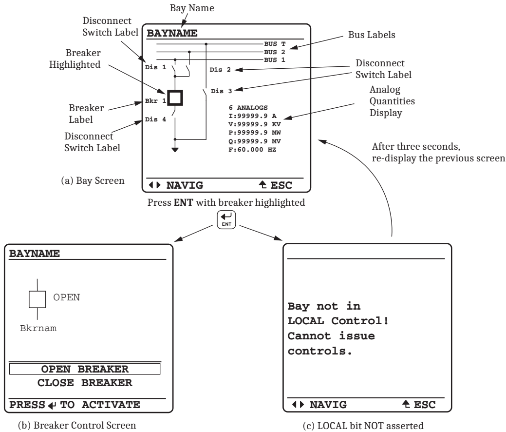
Figure 16 Screens for Circuit Breaker Selection
