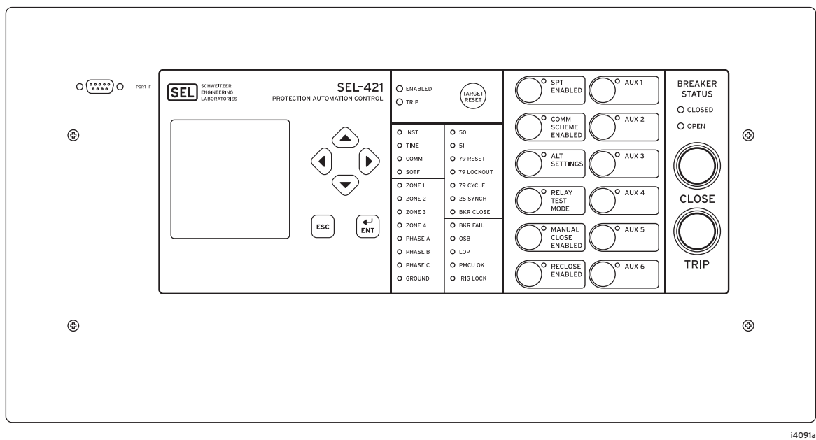
Figure 26 5U Front Panel, Panel-Mount Option With Extended HMI and Optional Trip/Close Pushbuttons
