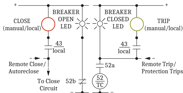
Figure 20 Optional Breaker Trip/Close Control Switches and Indicating Lamps
