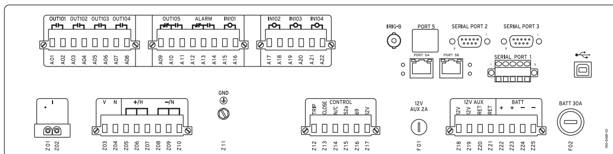
Figure 15 SEL-351RS Kestrel Side Panel
