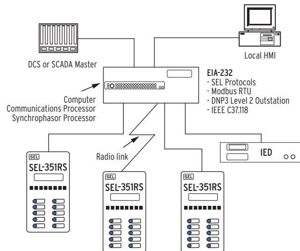
Figure 7 Typical Serial Communications Architecture
