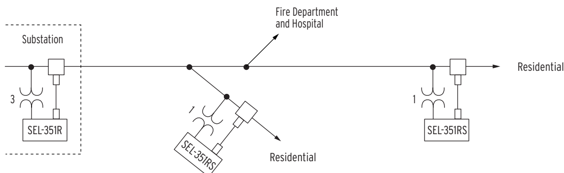
Figure 13 Implement Underfrequency Load Shedding With SEL-351RS Kestrel Recloser Controls to Preserve Critical Loads
