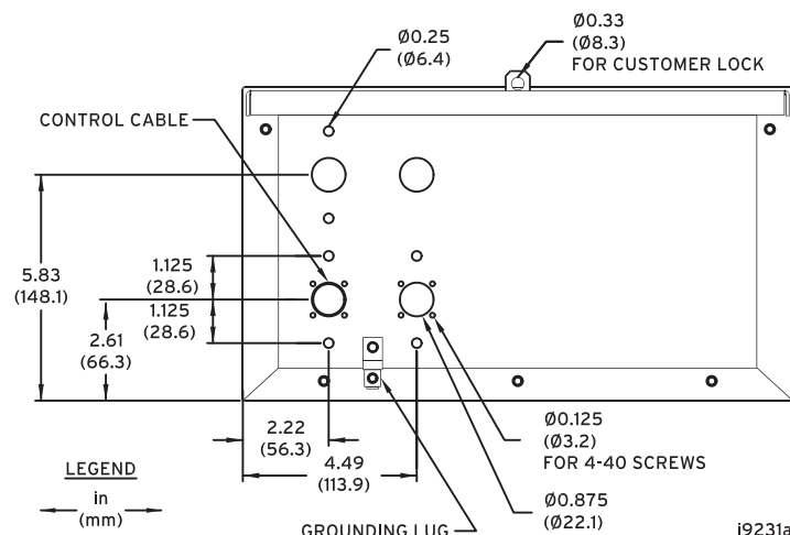
Figure 19 SEL-351RS Kestrel Lift-to-Open Enclosure Dimensions and Mounting
