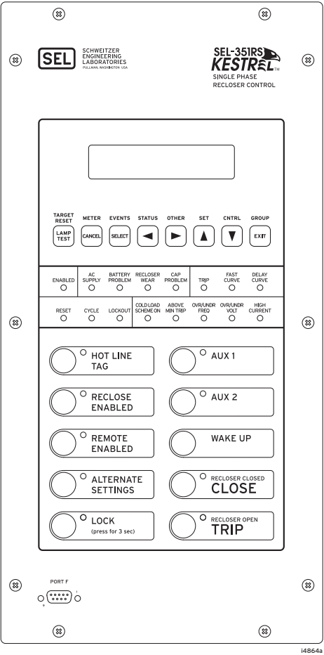
Figure 16 SEL-351RS Kestrel Recloser Control Front-Panel Interface
