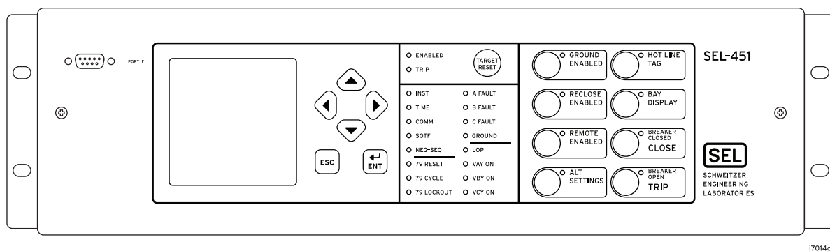
Figure 22 3U Front Panel, Rack-Mount Option With Standard HMI and Optional Bay Control Overlay
