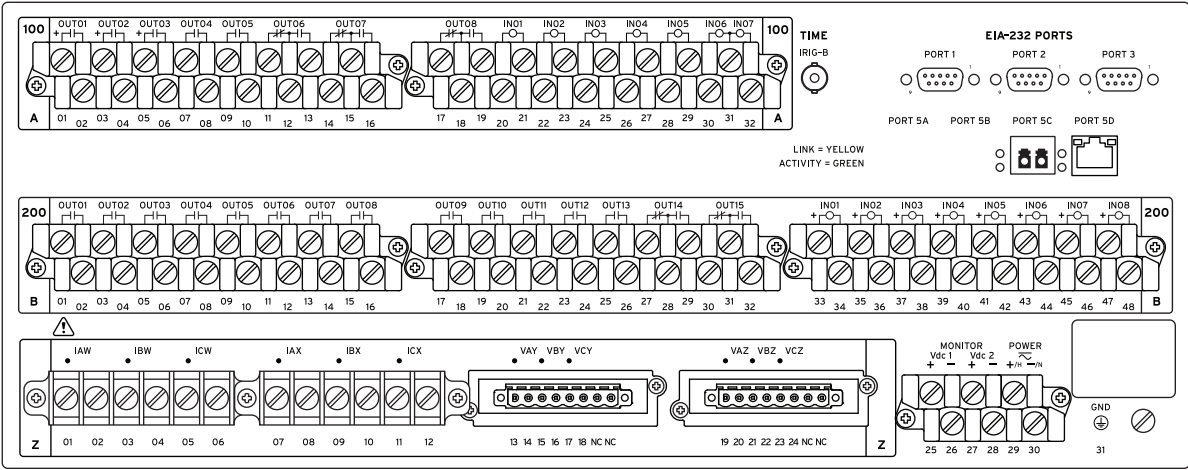
Figure 26 4U Rear Panel, Main Board, LEA Voltage Option With One (INT1) I/O Board
