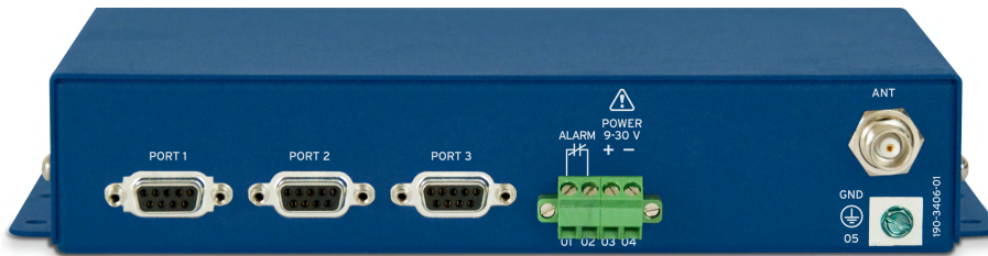
Figure 15 SEL-3031 Wall-Mount Rear Panel
