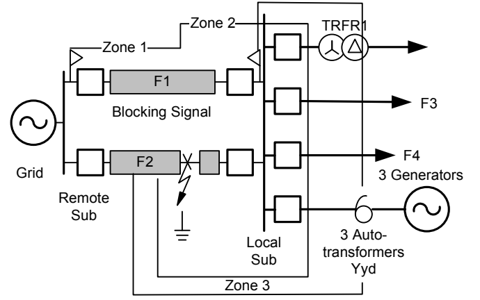
Fig. 1. Local network configuration
