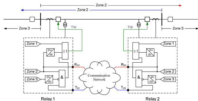
Fig. 22. A simplified sketch of a POTT communications-assisted tripping scheme
