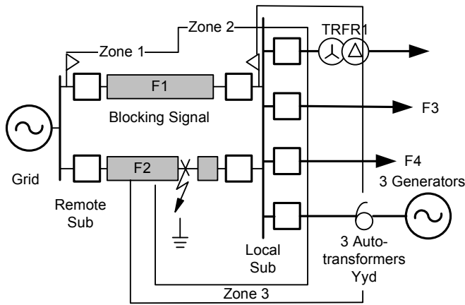
Fig. 29. Allocation of distance zones for DCB scheme on Feeder 1
