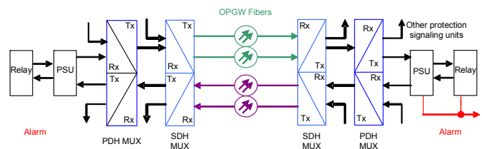
Fig. 43. A simplified sketch of a SDH and PDH system and teleprotection signals
