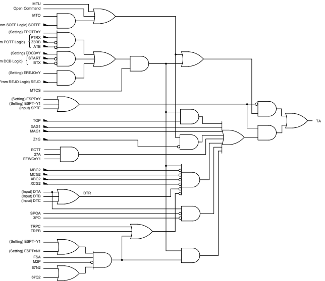
Fig. 11. Detailed tripping logic for a numerical distance relay (A-phase shown only)
