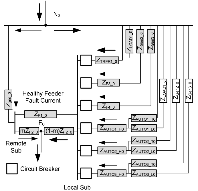
Fig. 1. Local network configuration
