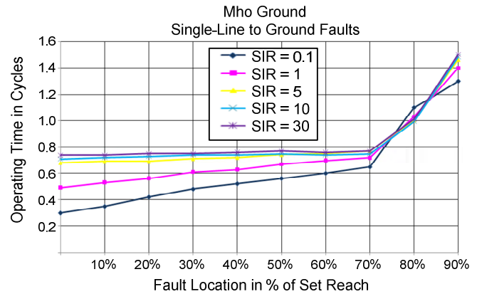
Fig. 35. Performance of a delta mho ground distance element over SIR range 0.1 to 30 ( Note: reach is limited to 70%)
