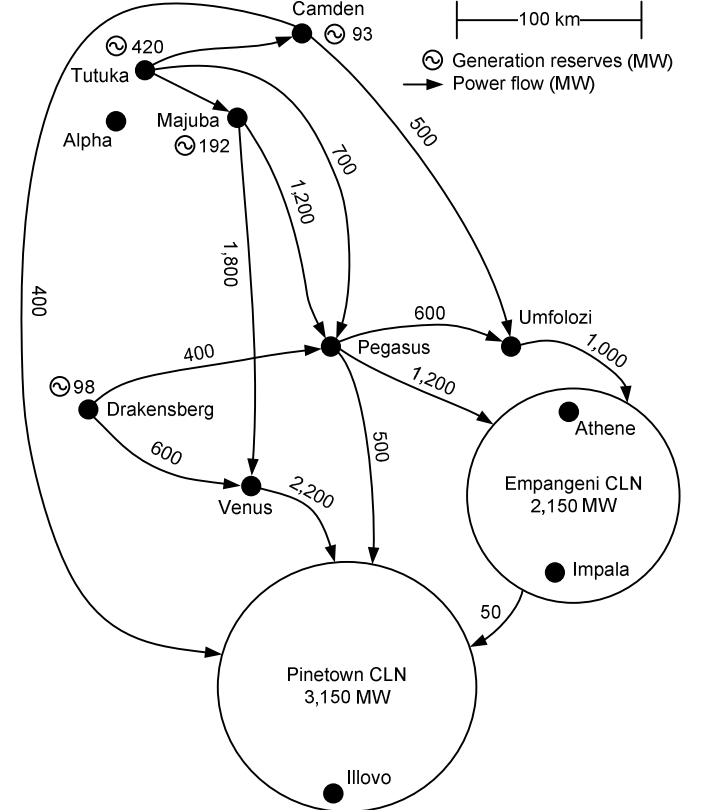
Fig. 4. Generation reserves and power flow in the Natal network, Pinetown CLN, and Empangeni CLN
