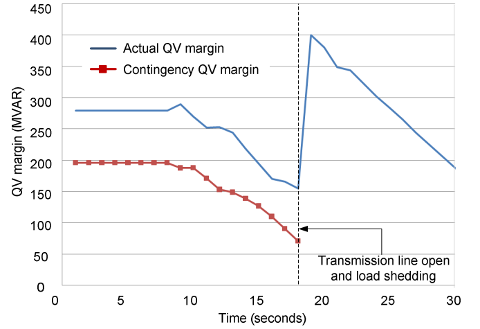
Fig. 16. SIPS restores the QV margin instantaneously after the contingency
