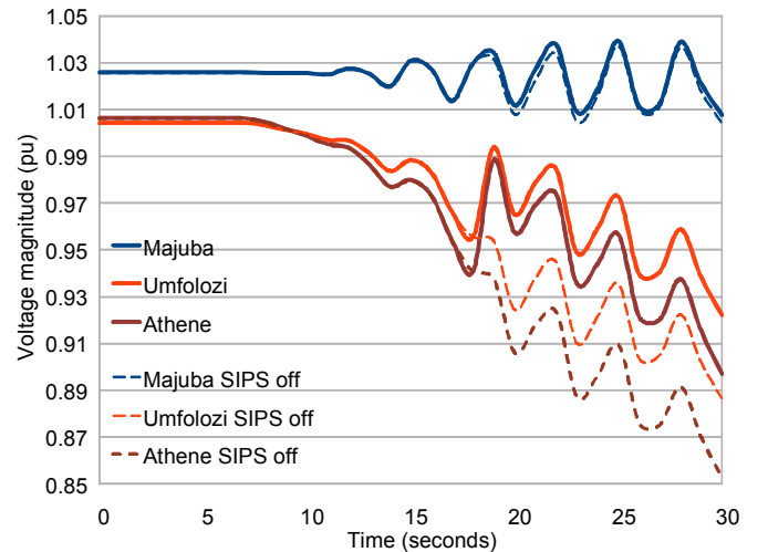
Fig. 17. Voltage magnitude recovers for 3 seconds after the SIPS sheds load
