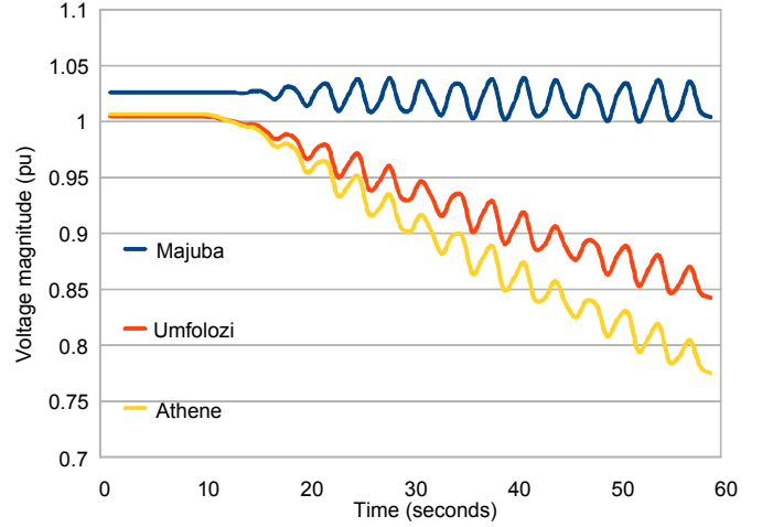
Fig. 8. Behavior of the voltage magnitudes for a constant increase in Q of 16 MVAR/s
