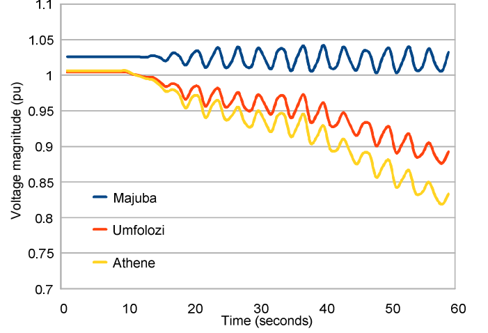
Fig. 12. Behavior of the voltage magnitudes for a constant increase in Q of 16 MVAR/s and automatic load shedding
