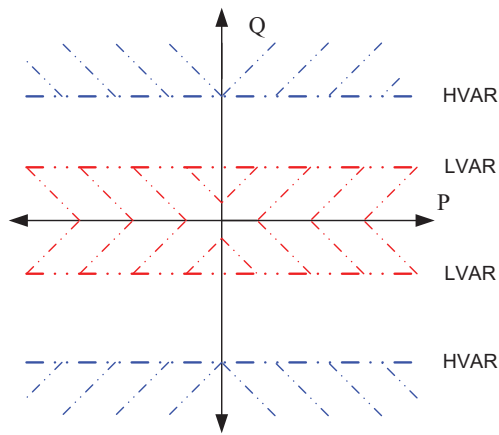
VAR deadband control characteristics.
