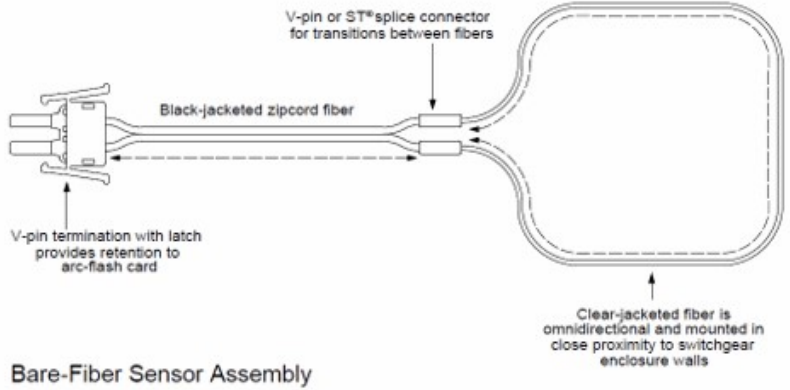
Figure 1 - Bare-Fiber Sensor Assembly with two splices
