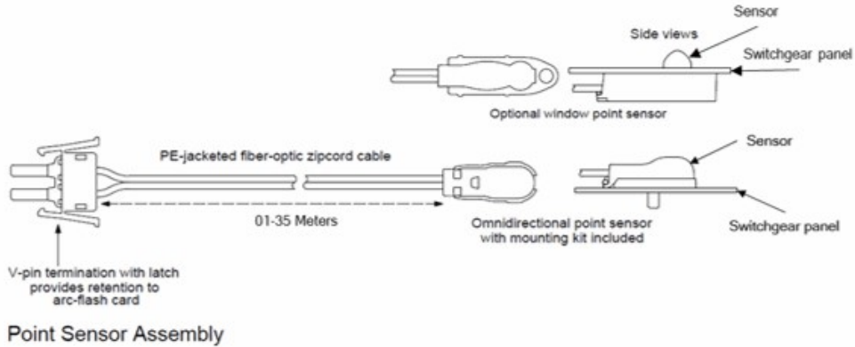
Figure 2 - Window Point Sensor (top) and Standard Point Sensor (bottom) Assemblies
