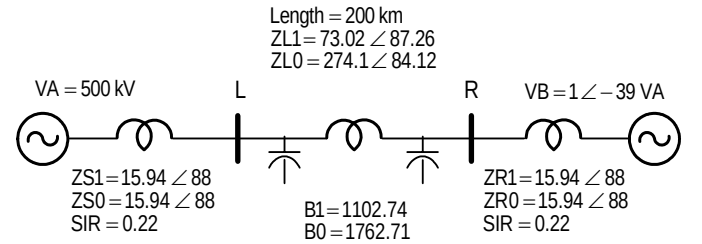
Fig. 17. 200 km 500 kV long line model
