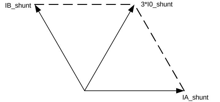
Fig. 12. Zero sequence current during a pole-open B
