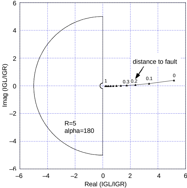
Fig. 6. 87LG element trajectories for an A-phase to-ground fault at different locations
