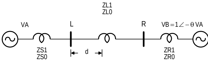
Fig. 27. Single-line network
