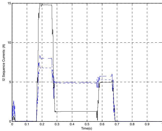
a) Negative-sequence currents
