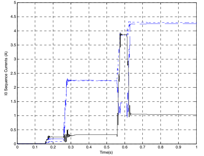
a) Zero-sequence currents
