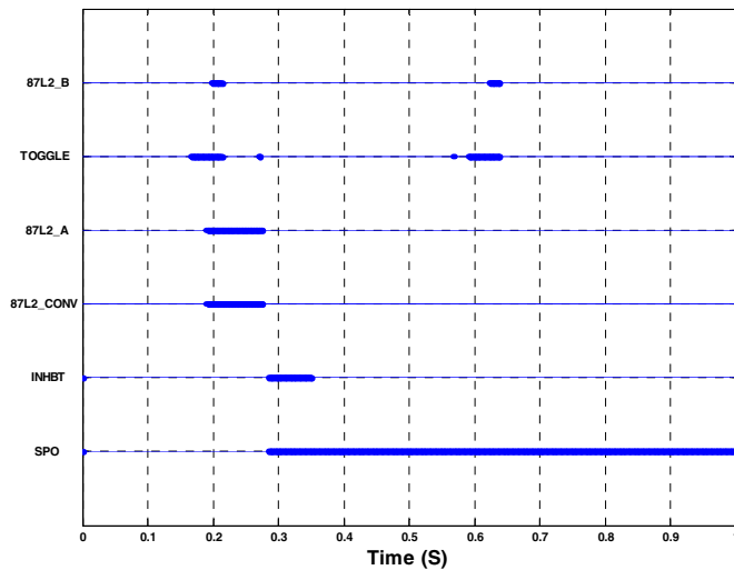
b) Logic signals
