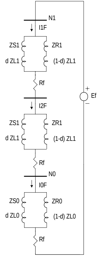
Fig. 28. A-phase-to-ground fault at R pure-fault sequence network
