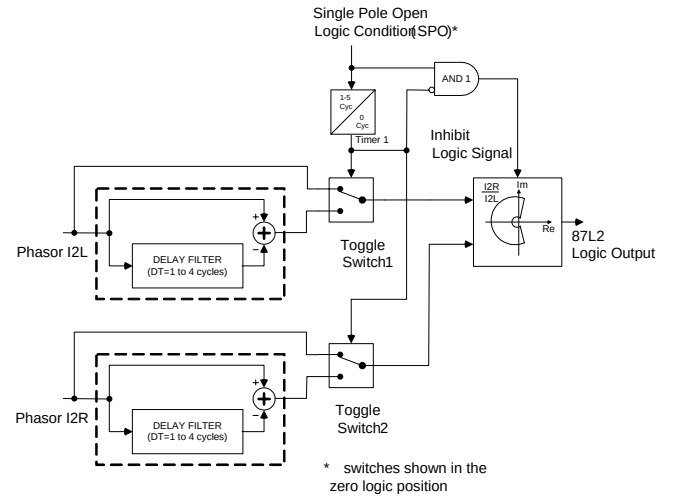
Fig. 14. Basic switch-compensated 87L2 element with conventional delta filters
