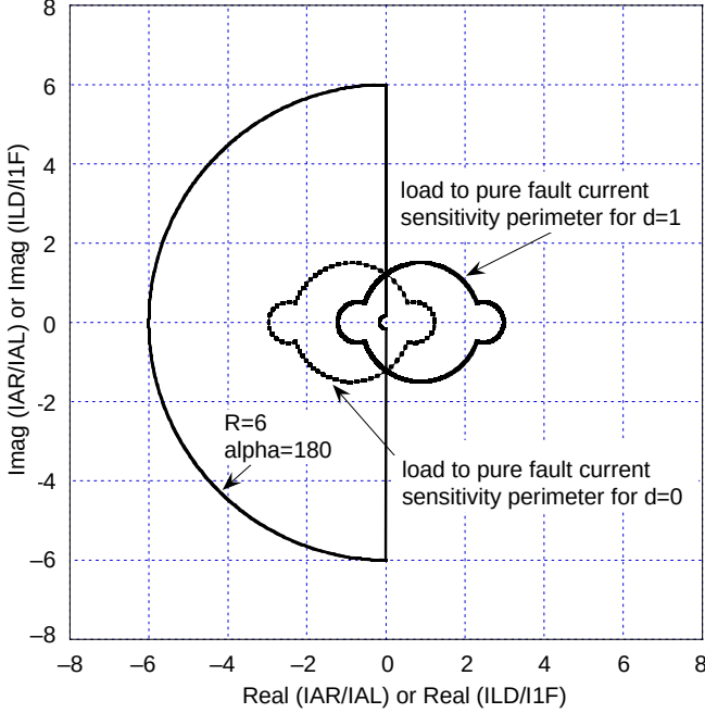
Fig. 4. Load-to-pure-fault current ratio sensitivity perimeter for phase-A-to-G faults
