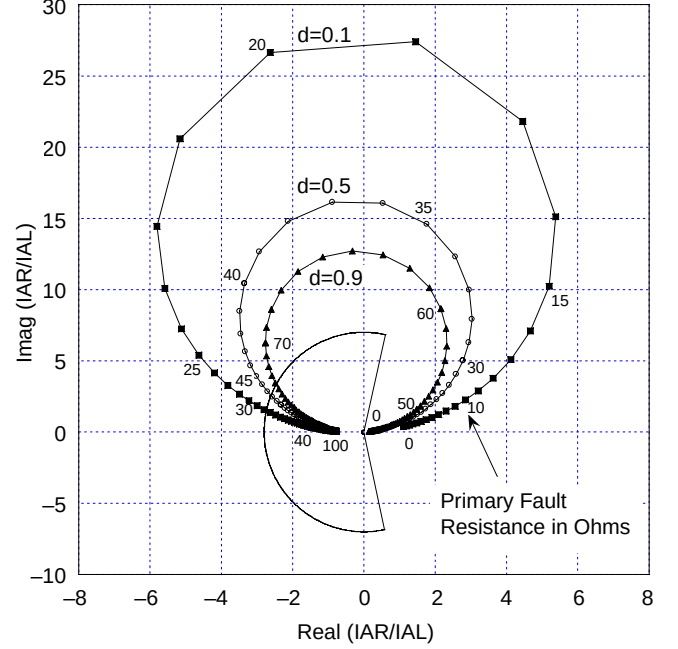
Fig. 5. 87LA element trajectories for an A-phase-to-G fault at three locations and variable fault resistance ( d expresses the fault location in per unit of line length)
