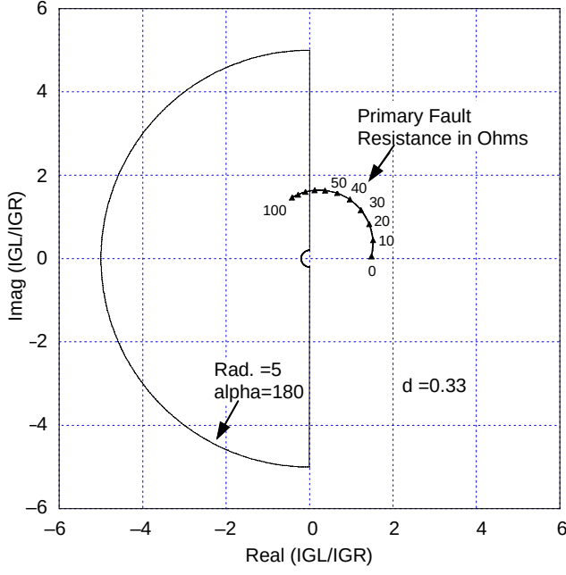
Fig. 7. 87LG element trajectory during a B-phase open with an A-phase-to-G fault with varying fault resistance
