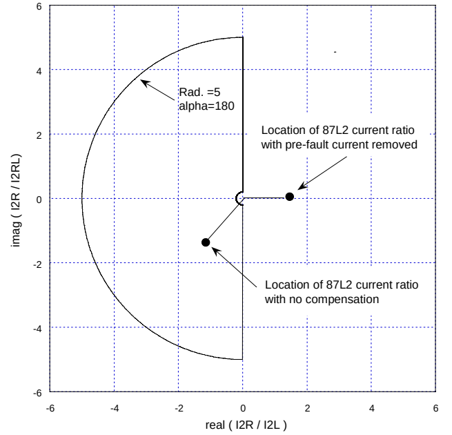
Fig. 9. 87L2 element current ratio loci during a B-phase open with an A-phase-to-G fault with prefault current present and removed
