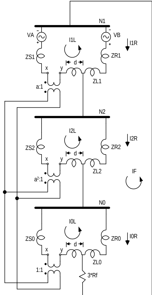
Fig. 30. Sequence network of B-phase open with A-phase-to-ground fault element in any network
