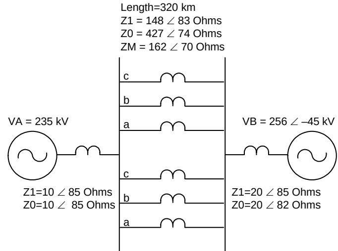
Fig. 22. 230 kV double-circuit line
