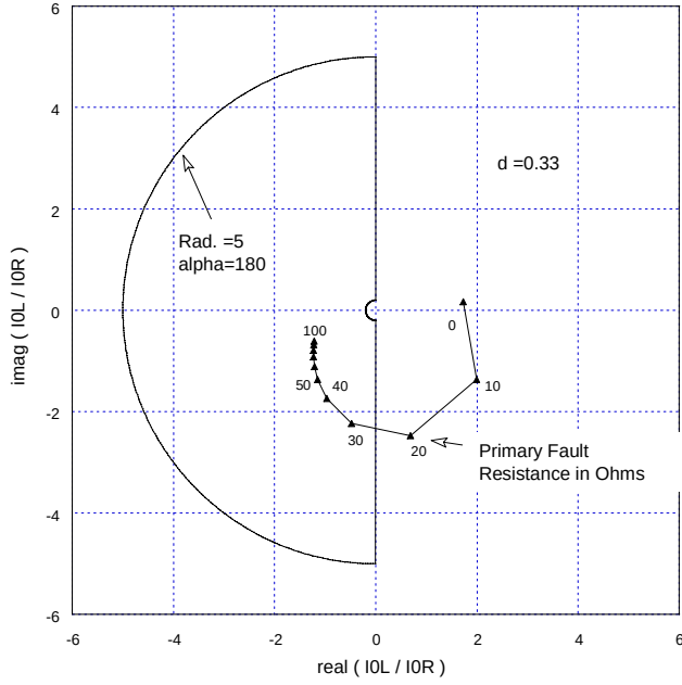
Fig. 8. 87L2 element trajectory during a B-phase open with an A-phase-to-G fault with varying fault resistance
