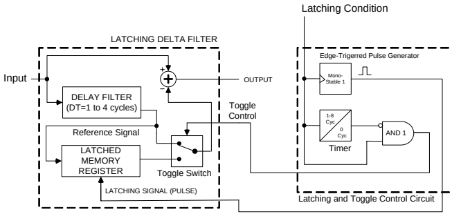
Fig. 11. The latching delta filter concept
