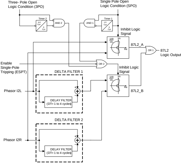
Fig. 15. Basic dual-compensated 87L2 element with conventional delta filters
