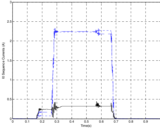
a) Zero-sequence currents
