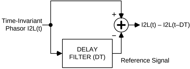
Fig. 10. Structure of a conventional delta filter
