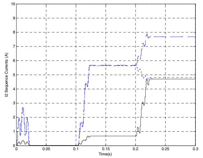
a) Negative-sequence currents
