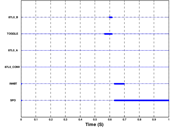
b) Logic signals
