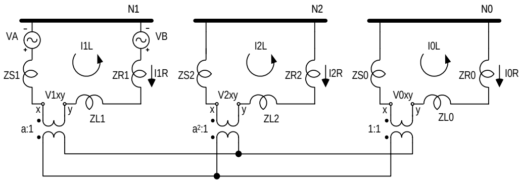
Fig. 29. Sequence network of B-phase open elementary network
