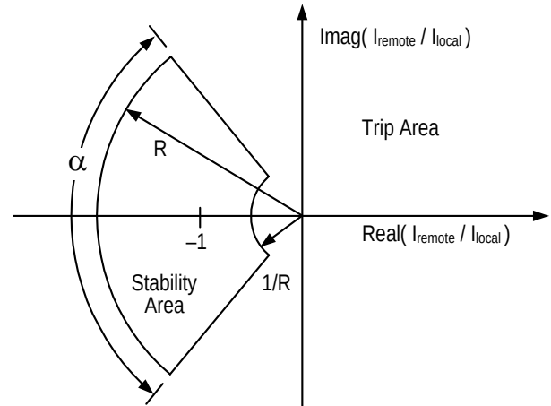
Fig. 1. Differential Element Characteristic Embedded in the Current-Ratio Plane
