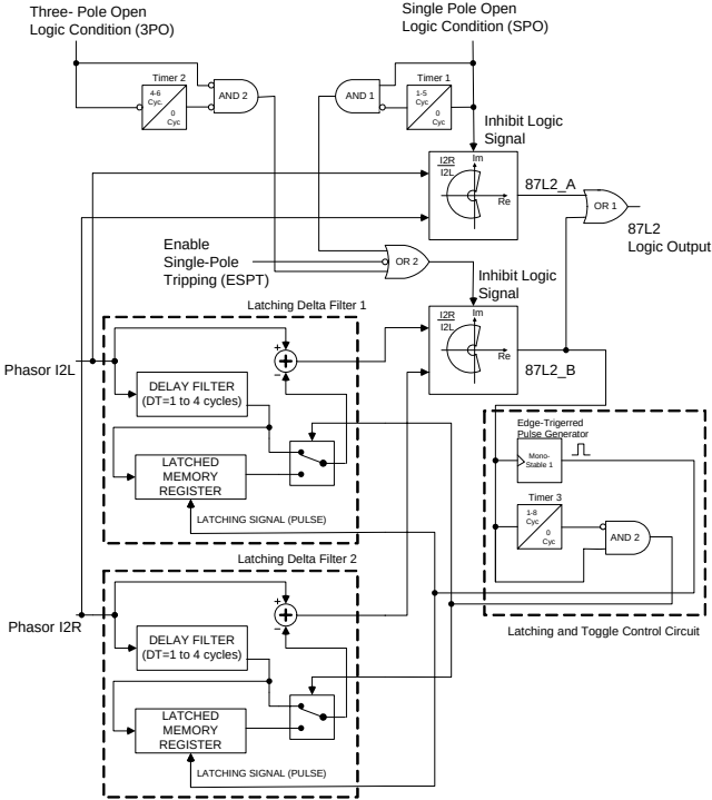
Fig. 16. Advanced dual-compensated 87L2 element with latching delta filters
