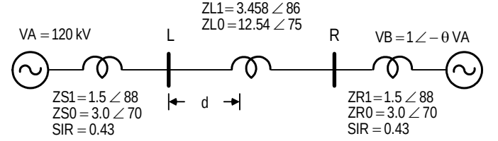
Fig. 3. 120 kV Elementary network
