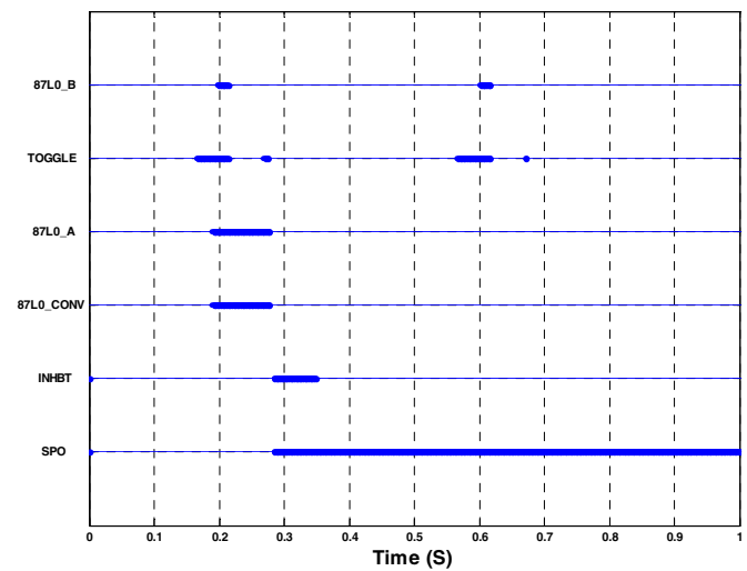
b) Logic signals
