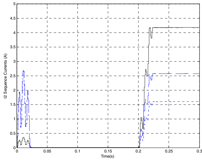
a) Negative-sequence currents
