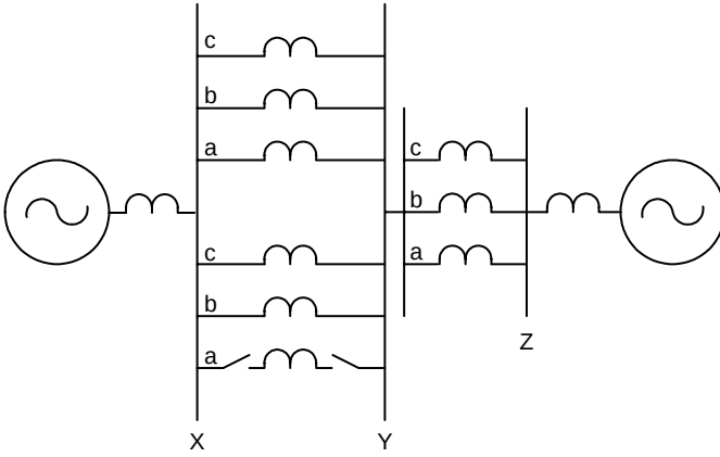
Fig. 13. Impact of a pole open on adjacent lines
