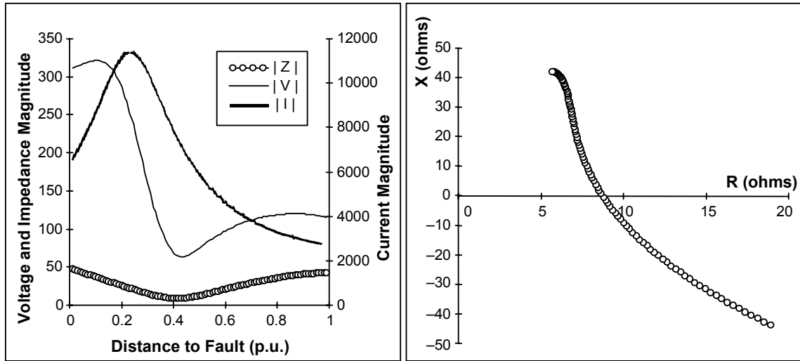
Figure 11 Measurement values by Pegasus-Umfolozi impedance relay for faults, at various distances, on the Umfolozi-Athene 400 kV feeder during maximum fault conditions
