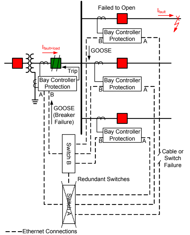
Fig. 15. Breaker Failure Scheme in the Case of Cable or Ethernet Switch Failure
