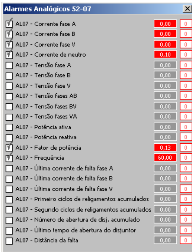
Fig. 10. Feeder Analog Measurements
