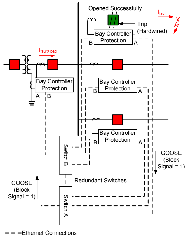
Fig. 18. GOOSE Message to Block the Fast Overcurrent Element of the Incoming Feeder
