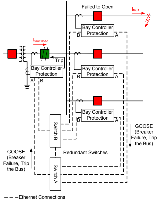
Fig. 14. Breaker Failure Implementation Using GOOSE Messages
