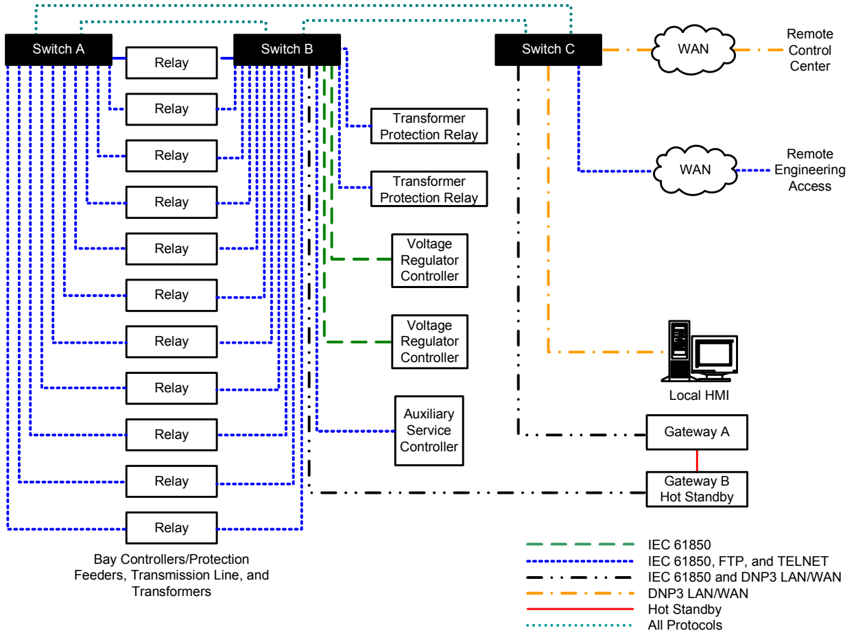
Fig. 3. Network Architecture Adopted for the Automation System
