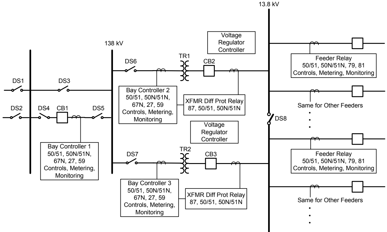
Fig. 2. Distribution of the IEDs in the Bays
