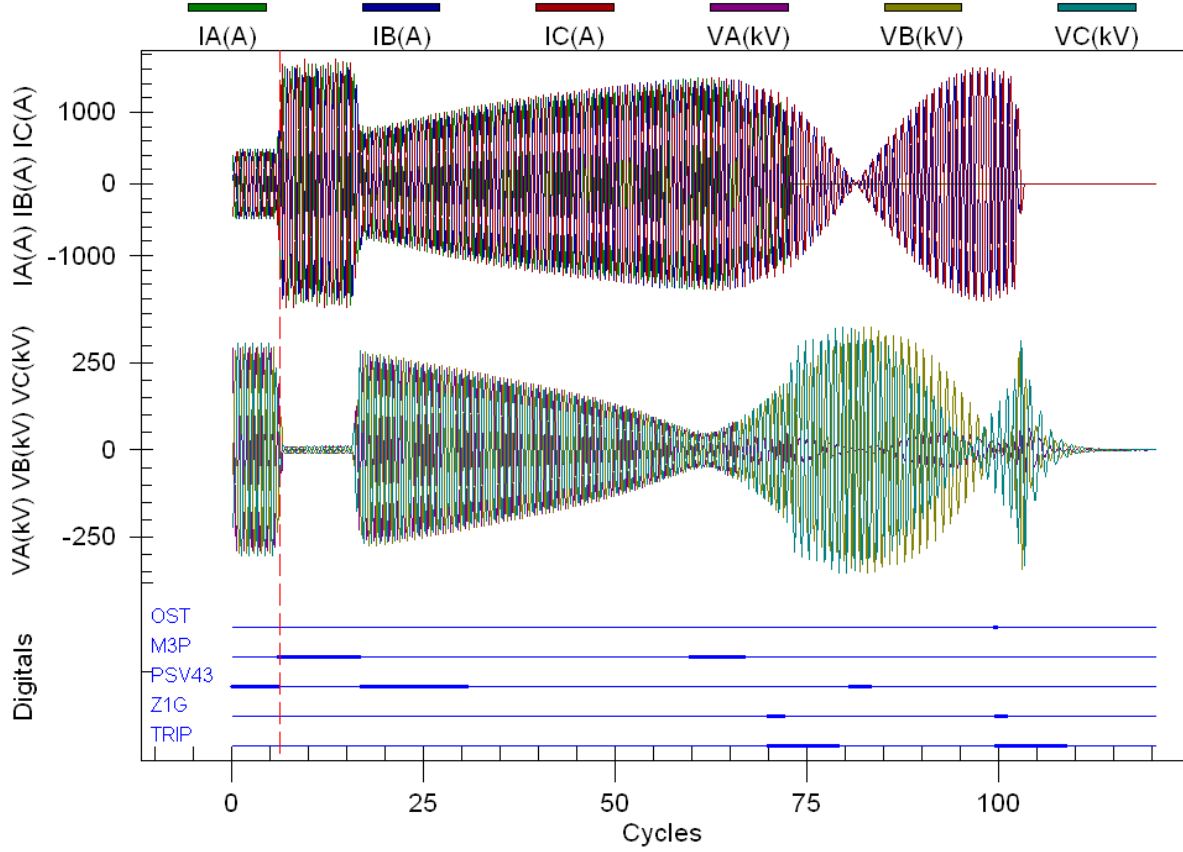
Fig. 11. SKA Protection System Response for an AG Fault During the Swing
