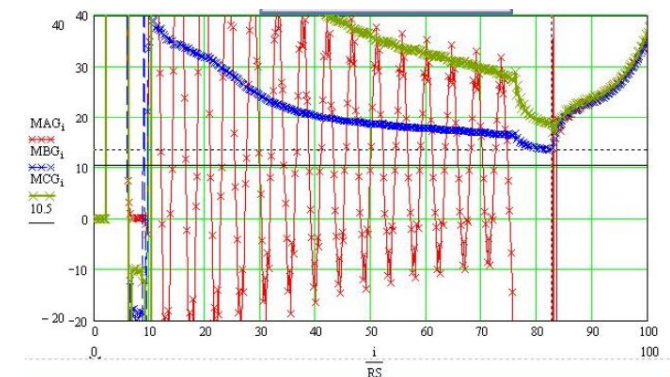
Fig. 18. SEL Ground Elements for an AG Fault on 5L96, With RAS
