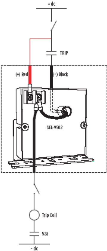
Typical SEL-9502 Contact Arc Suppressor Application (280 Vdc Maximum)
