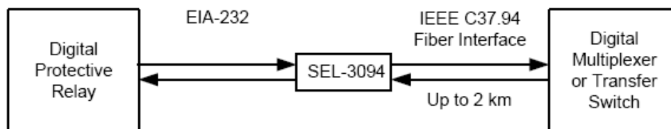
Figure 2. The SEL-3094 interfaces EIA-232 relays to multiplexers and switching equipment.
