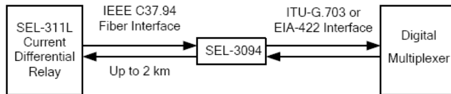
Figure 1. The SEL-3094 connects IEEE C37.94 compliant relays with non-compliant digital multiplexers.
