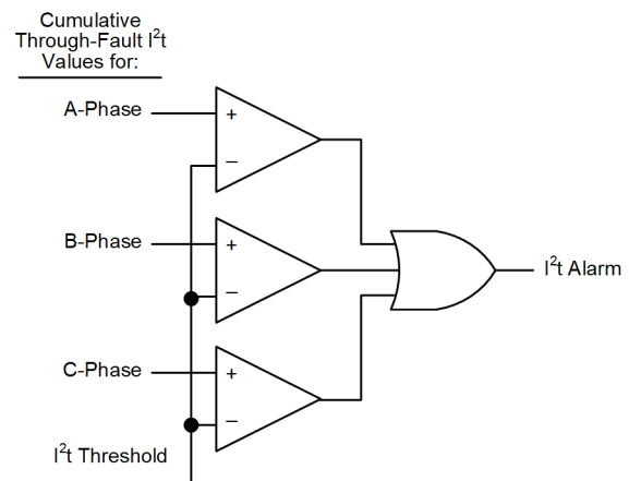
Fig. 9. Cumulative Through-Fault Logic
