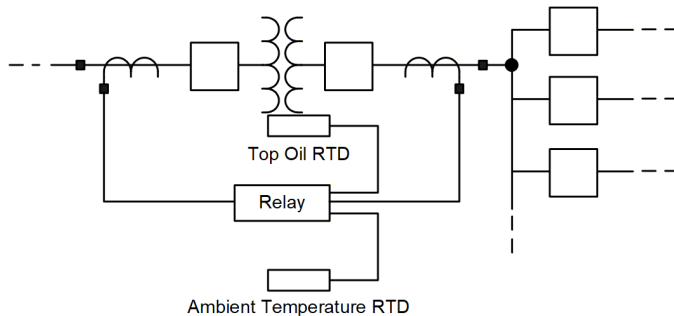
Fig. 7. Transformer Protection Relay With Connected RTDs for Thermal Monitoring
