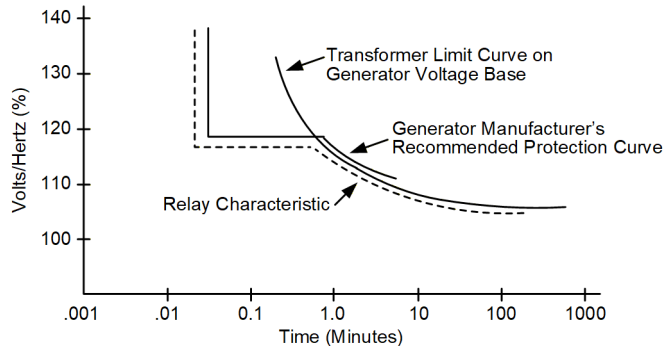
Fig. 12. Overexcitation Protection Coordination Curve
