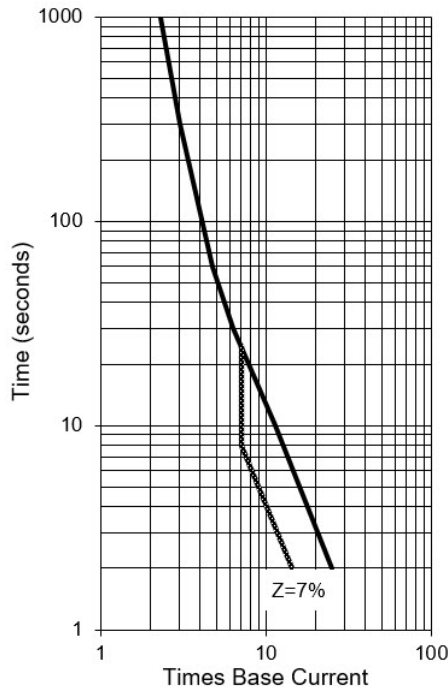
Fig. 4. Through-Fault Capability Limit Curve for Liquid-Immersed Category IV Transformers
