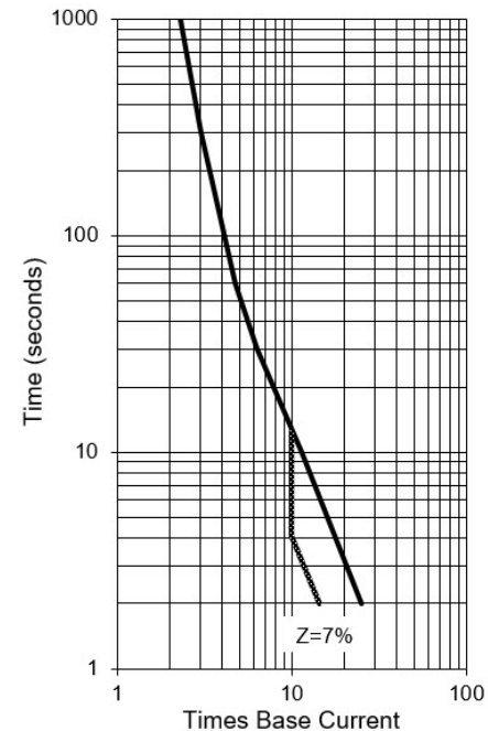
Fig. 3. Through-Fault Capability Limit Curve for Liquid-Immersed Category II Transformers with Frequent Faults
