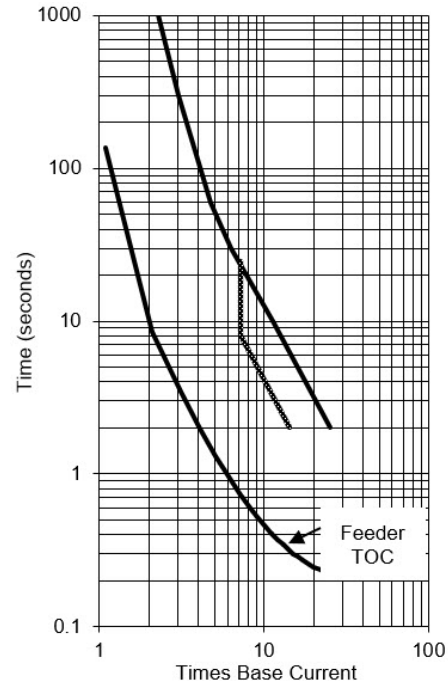
Fig. 5. TOC Coordination with Category IV Transformer Through-Fault Capability Limit Curve
