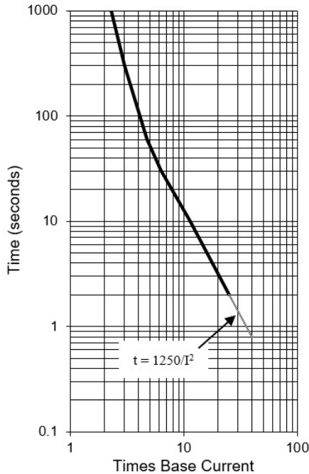
Fig. 1. Through-Fault Capability limit curve for Liquid-Immersed Category I Transformers
