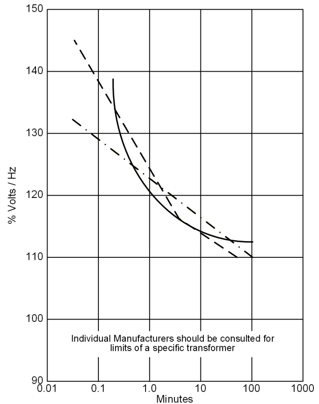
Fig. 11. Typical Transformer Overexcitation Limit Curves
