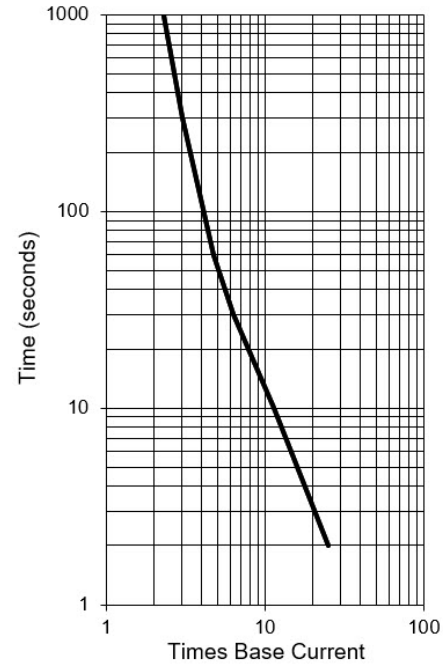
Fig. 2. Through-Fault Capability Limit Curve for Liquid-Immersed Category II and III Transformers with Infrequent Faults
