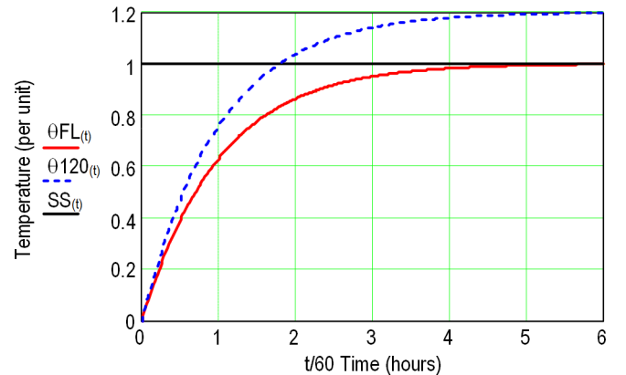
Fig. 6. Oil Temperature Curves For Full-Load Current and Twenty Percent Overload Current
