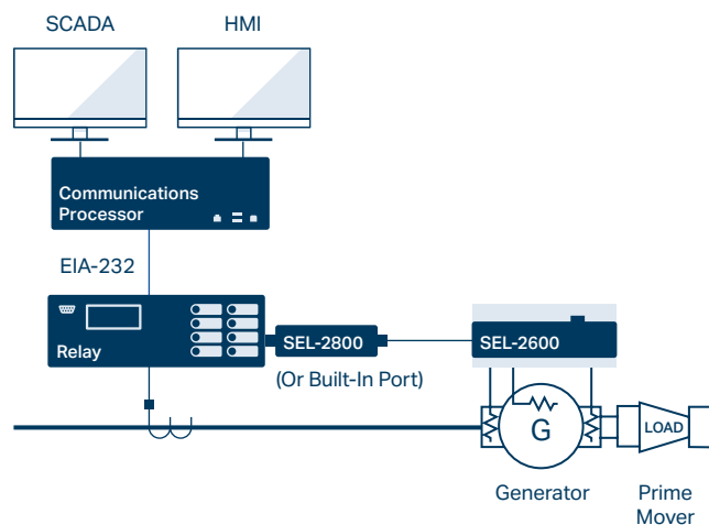
RTD thermal data transmitted to a relay.
