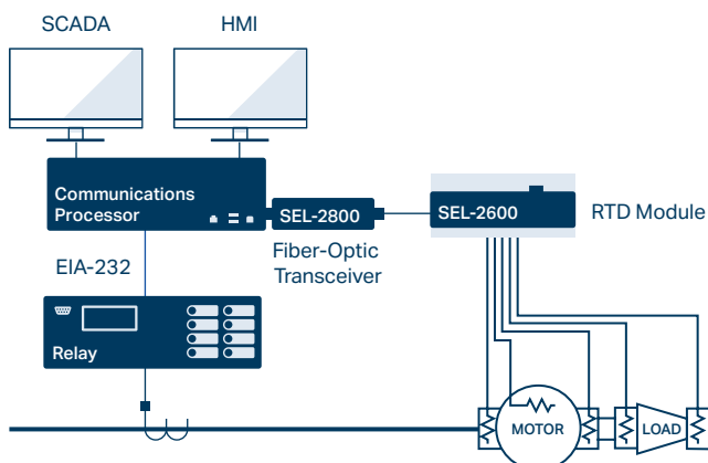
RTD thermal data transmitted to a communications processor.
