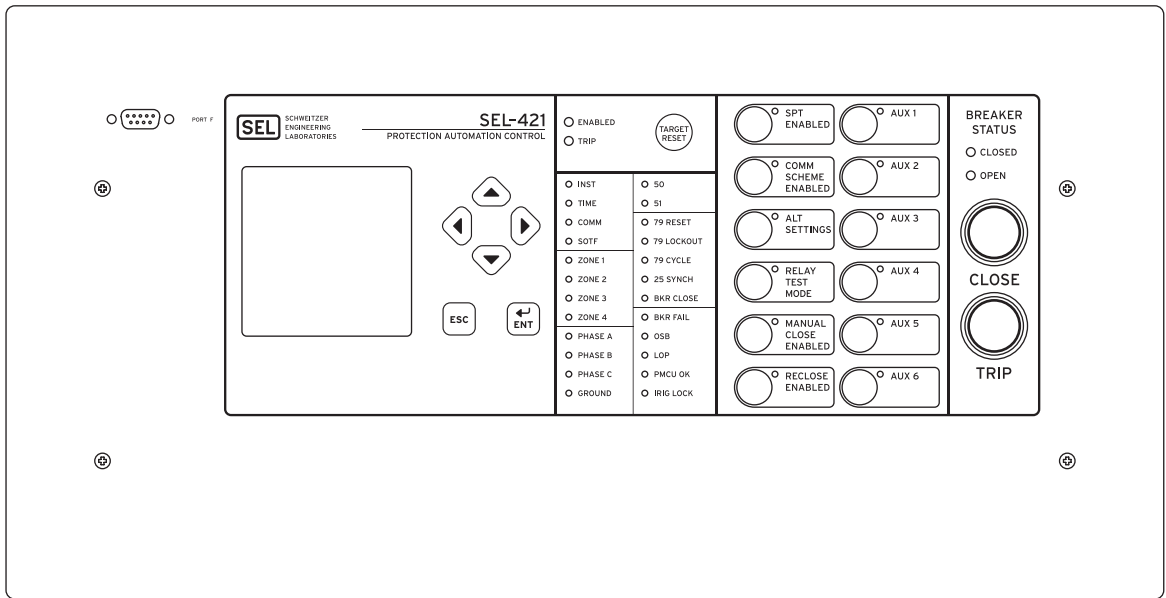
Figure 22 Typical SEL-421 Front-Panel Diagrams
