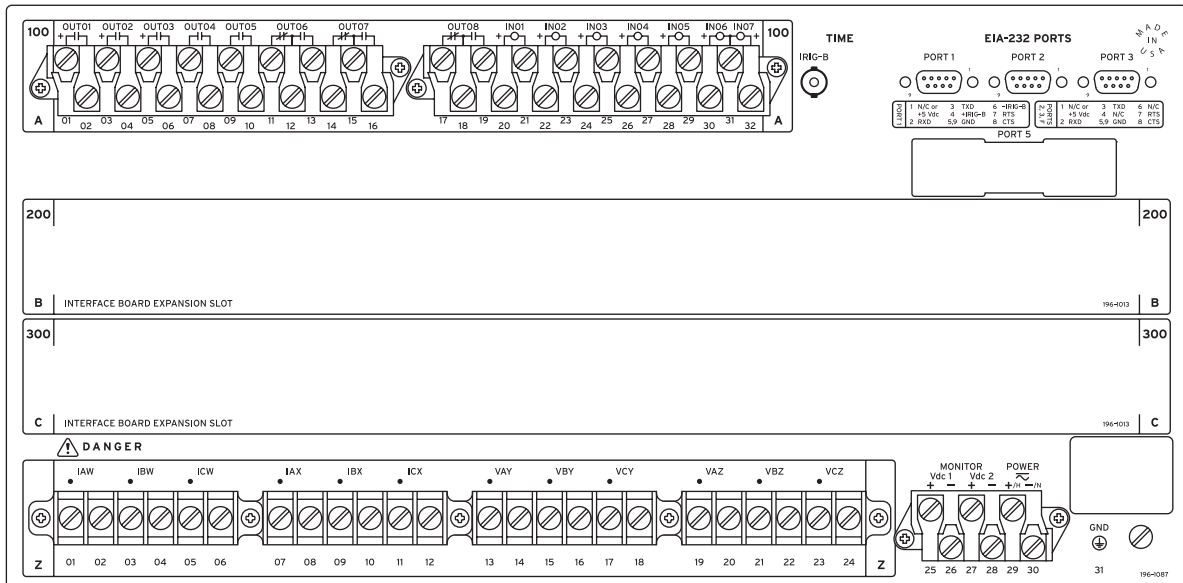
5U Rear Panel, With Space for Additional I/O Boards
