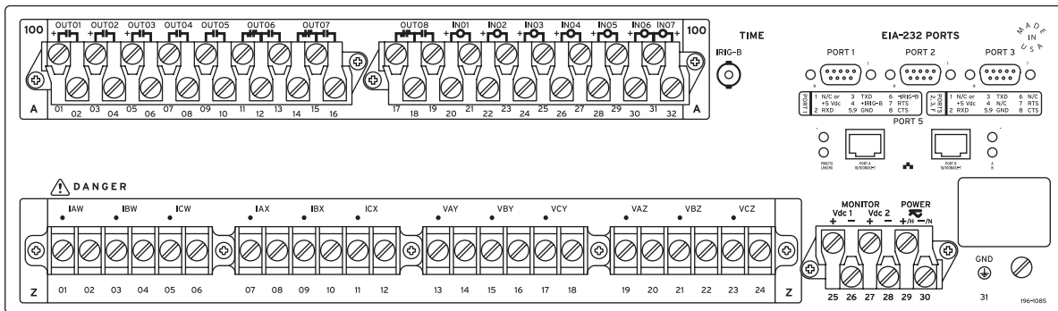
3U Rear Panel, Main Board A
