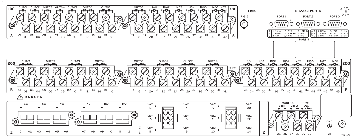
4U Rear Panel, Main Board A, Connectorized® Option, INT5 I/O Board
