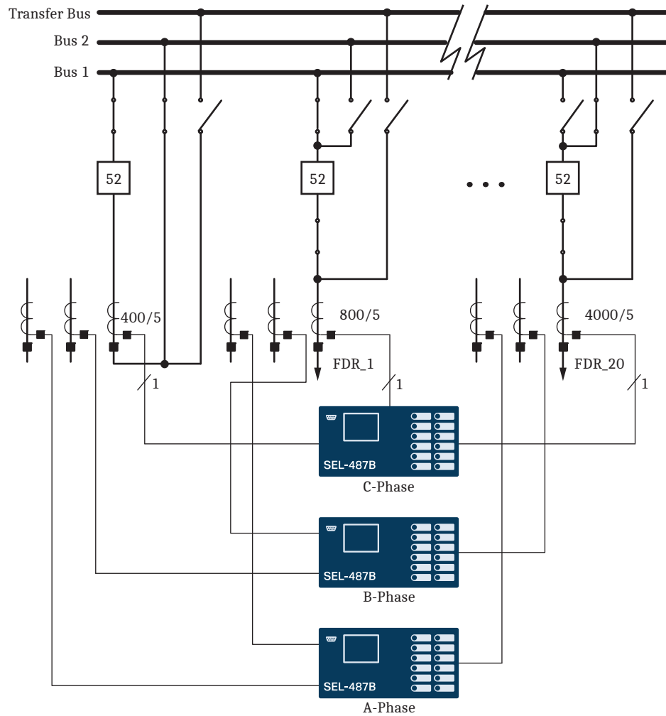
Figure 17 Three SEL-487B Relays Protect Two Main Busbars, a Transfer Busbar, Bus Coupler, and 20 Terminals
