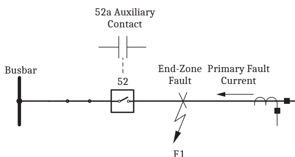
Figure 10 Bus Protection Is Not Affected by Fault, F1; Use Transfer Trip to Clear the Fault
