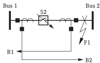
Figure 12 Two CTs Configured in Overlap
