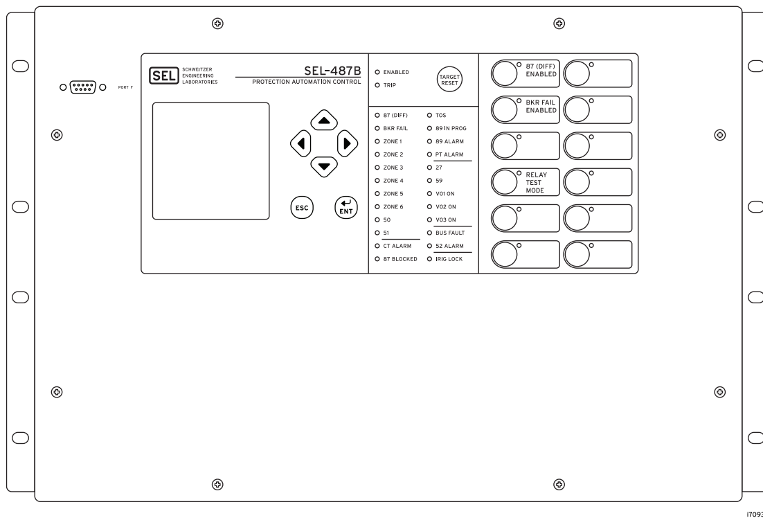
Figure 26 7U Front Panel, Rack-Mount Option
