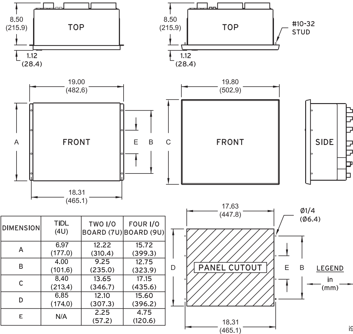
Figure 30 Dimensions for Rack- and Panel-Mount Models
