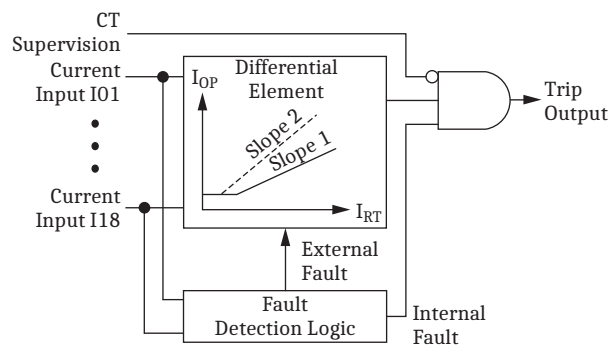
Figure 3 External Fault Detection Logic Increases Differential Element Security
