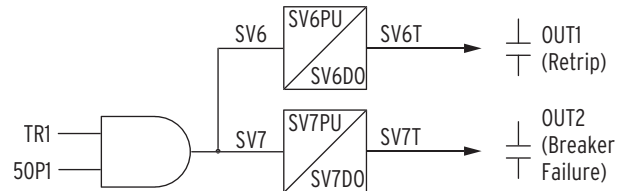
Figure 11 Dedicated Breaker Fail Scheme Created With SELogic Control Equation Variables/Timers
