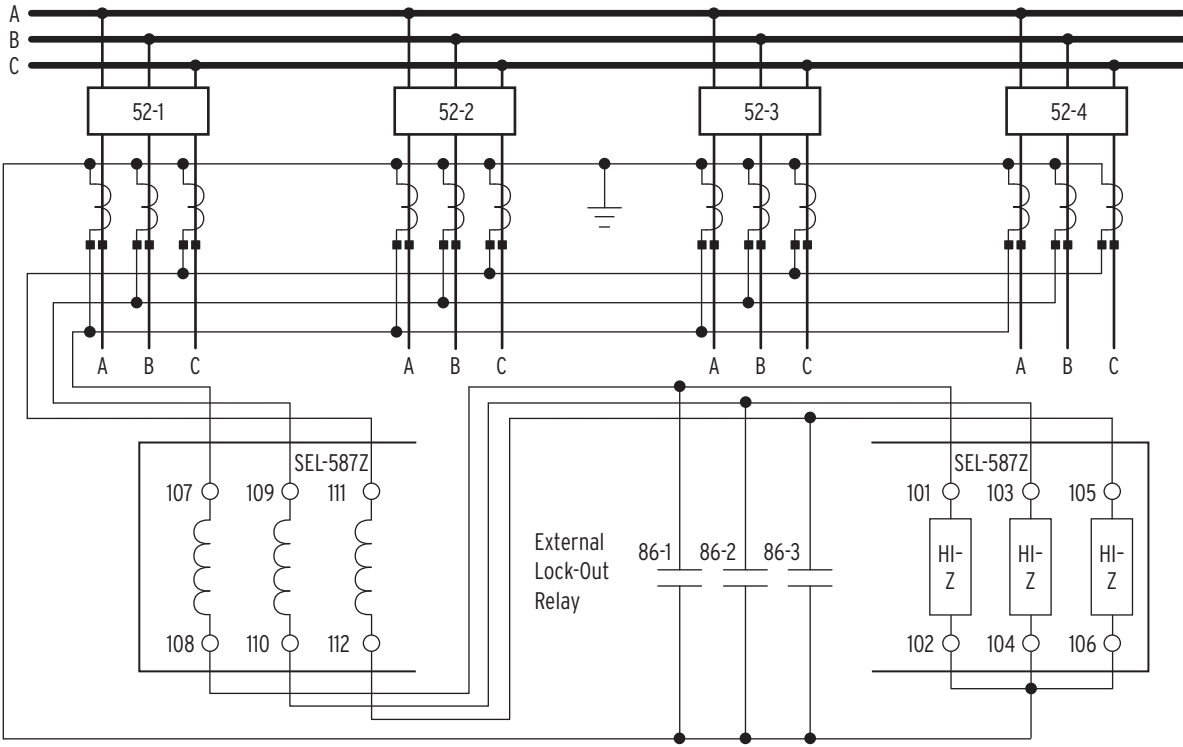
Figure 16 Example AC Connection With 50/51 Overcurrent Element
