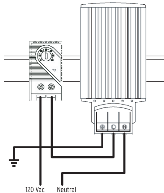
Figure 1 Diagram of Heater Accessory Connections
