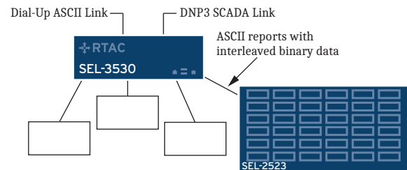
Figure 4 Example Communications System
