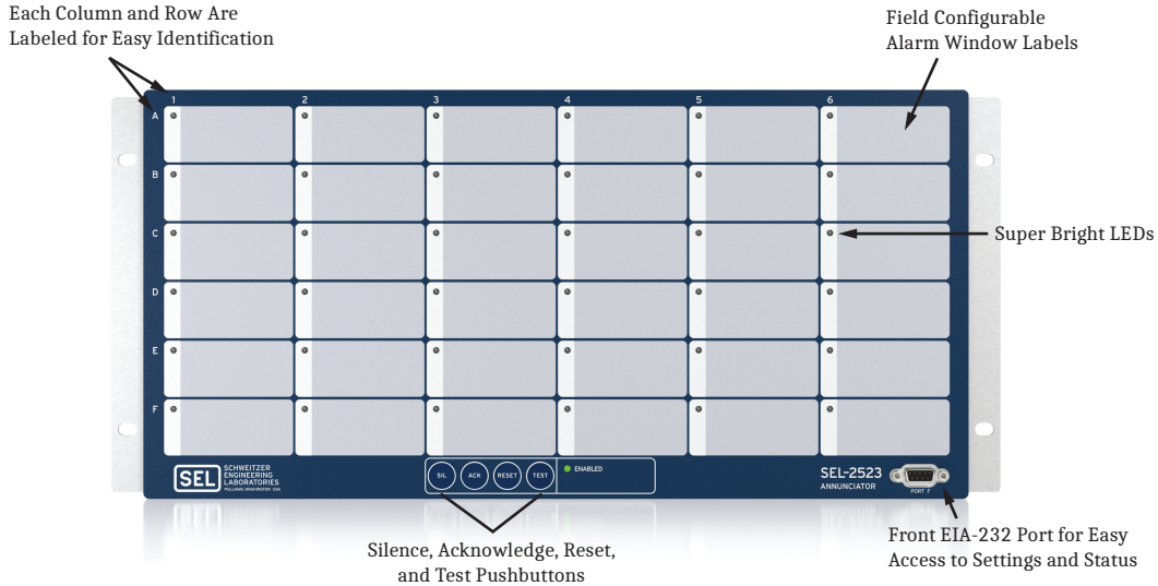
Figure 1 SEL-2523 Front View
