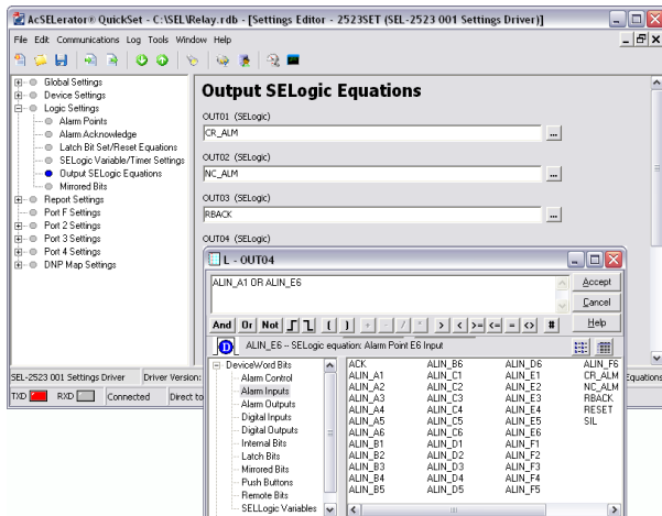
Figure 6 Create SELogic Control Equations With a Drag-and-Drop Editor and a Text Editor
