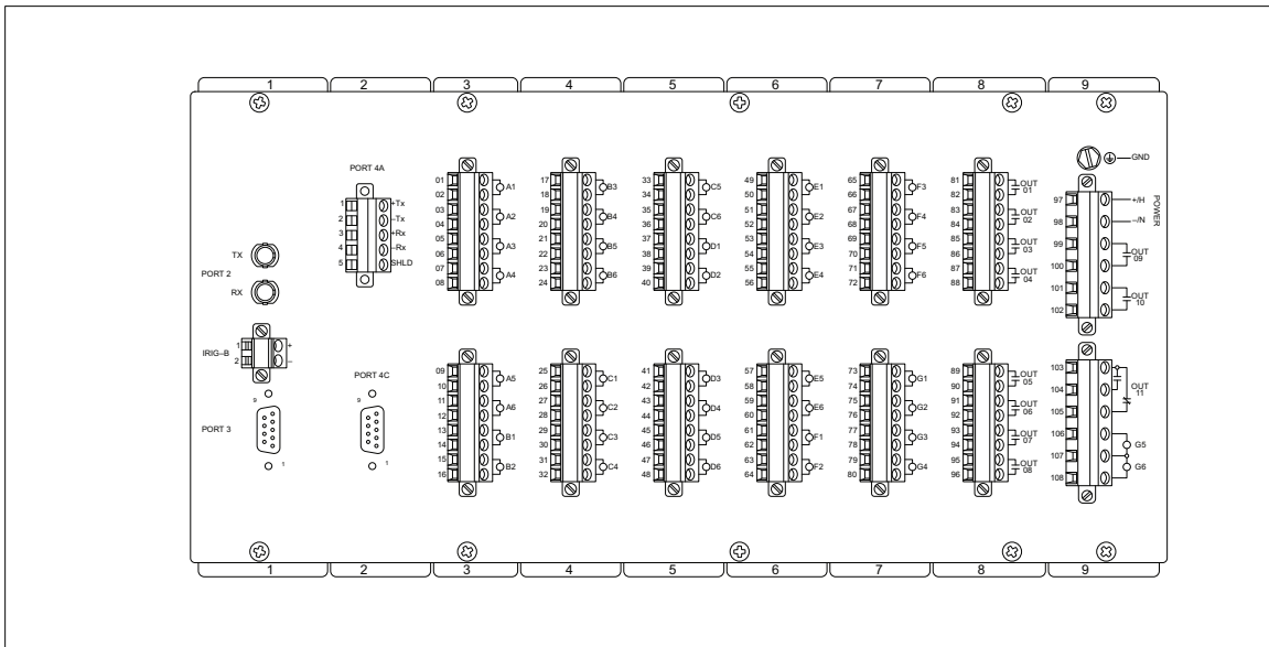
Figure 11 SEL-2523 Rear Panel
