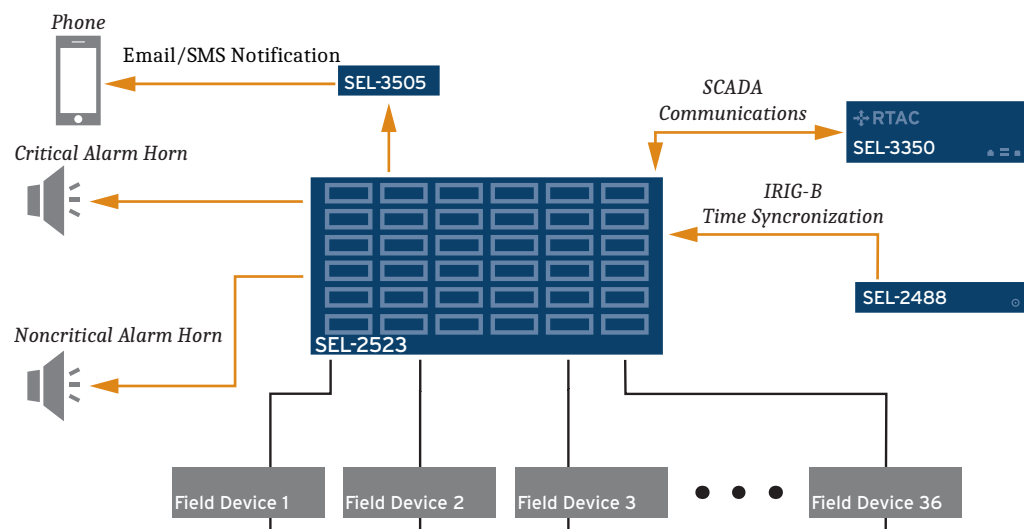
Figure 3 SEL-2523 Functional Diagram
