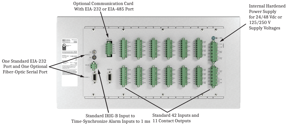
Figure 2 SEL-2523 Rear View
