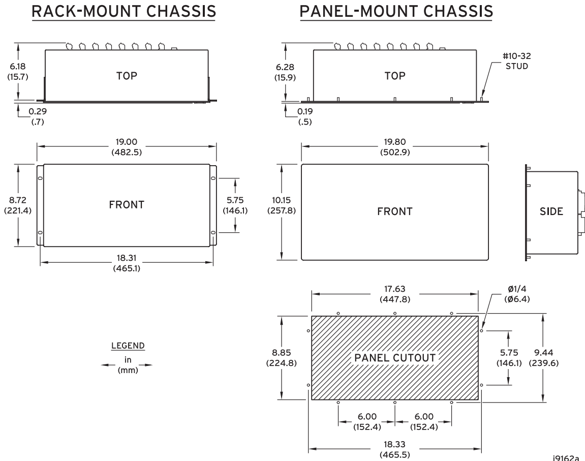
Figure 12 SEL-2523 Rack-Mount and Panel-Mount Chassis
