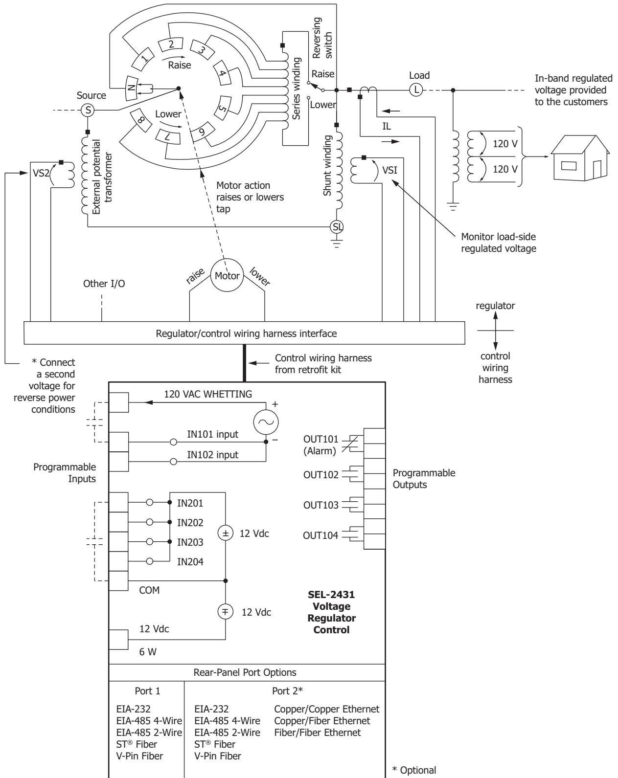
Figure 3 Functional Diagram
