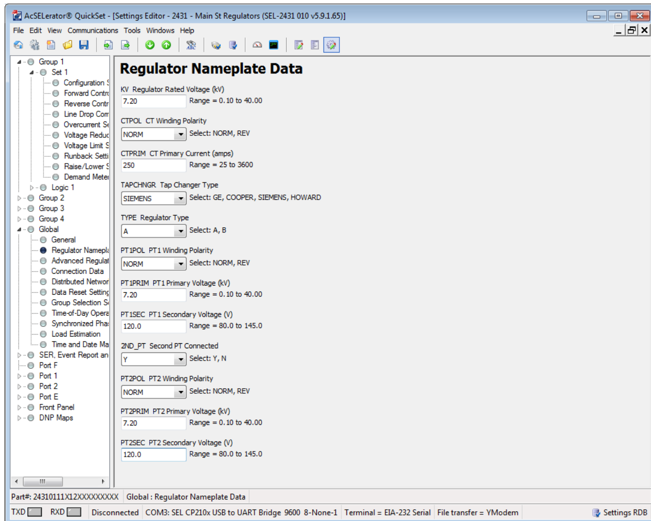
Figure 15 QuickSet Nameplate Data Screen
