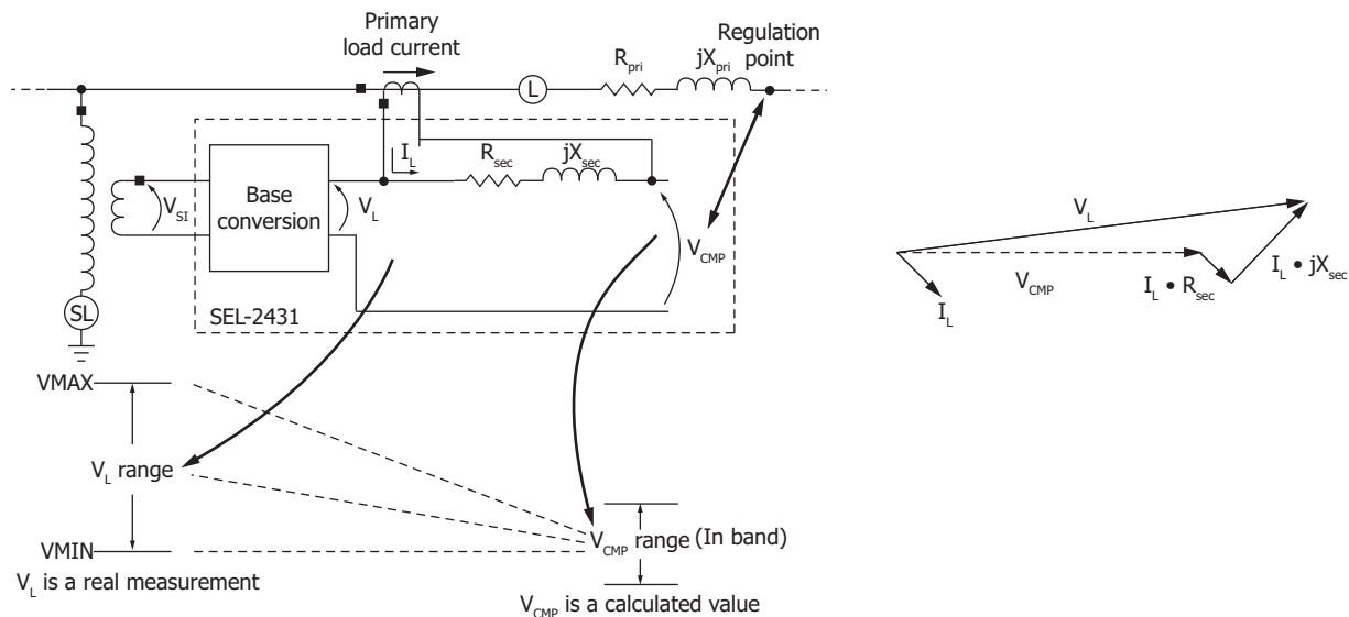
Figure 6 Line-Drop Compensation Keeps Voltage Constant at the Regulation Point
