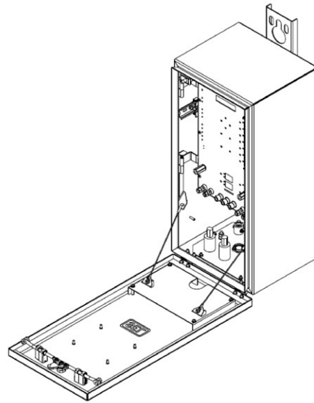
Figure 5 SEL-2431 Enclosure
