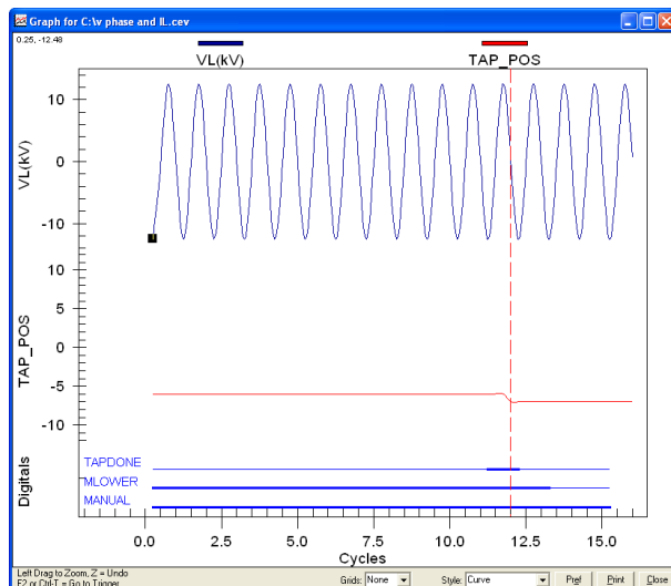
Figure 16 QuickSet Event Report
