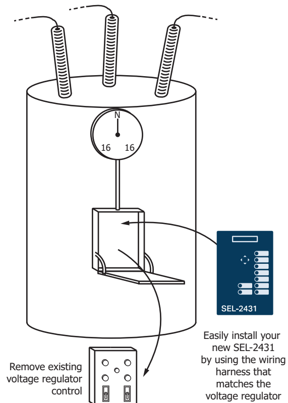
Figure 2 Voltage Regulator Control Retrofit With SEL-2431
