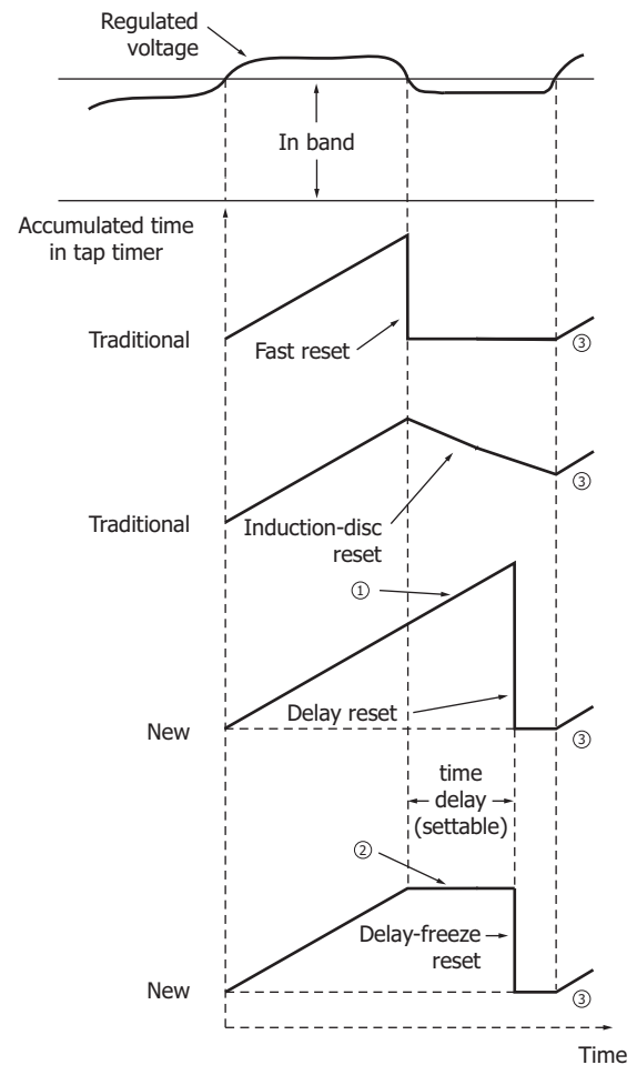
① Do not interrupt timing if in-band voltage excursion is less than a settable time delay. ② Temporarily “freeze” timing if in-band voltage excursion is less than a settable time delay. ③ Tap timer starts timing again when the in-band voltage excursion ends.
