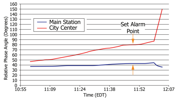
Figure 11 Visualization of Phase Angle Measurements Across a Power System
