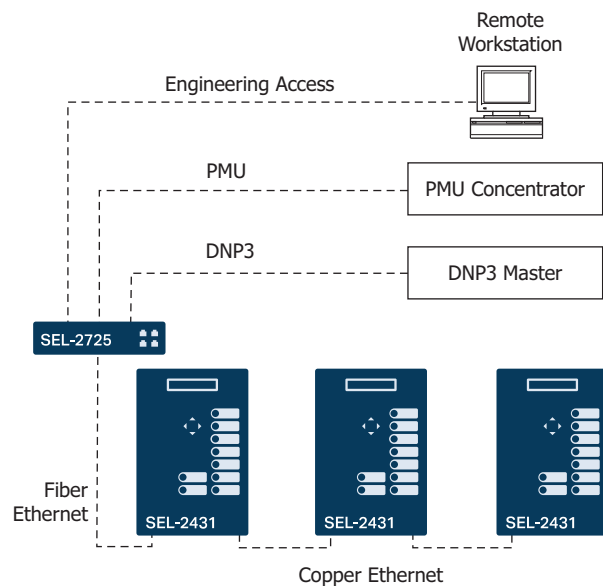
Figure 1 Ethernet-Connected Voltage Regulator Controls
