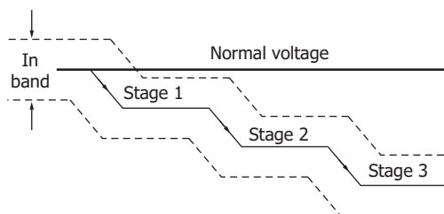
Figure 7 Set Up Three Voltage-Reduction Stages for System Stability Support
