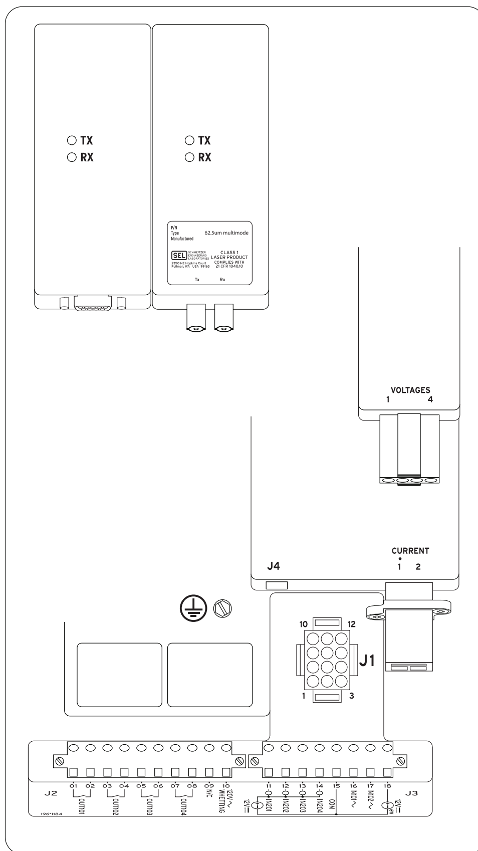
Figure 18 SEL-2431 Rear Panel
