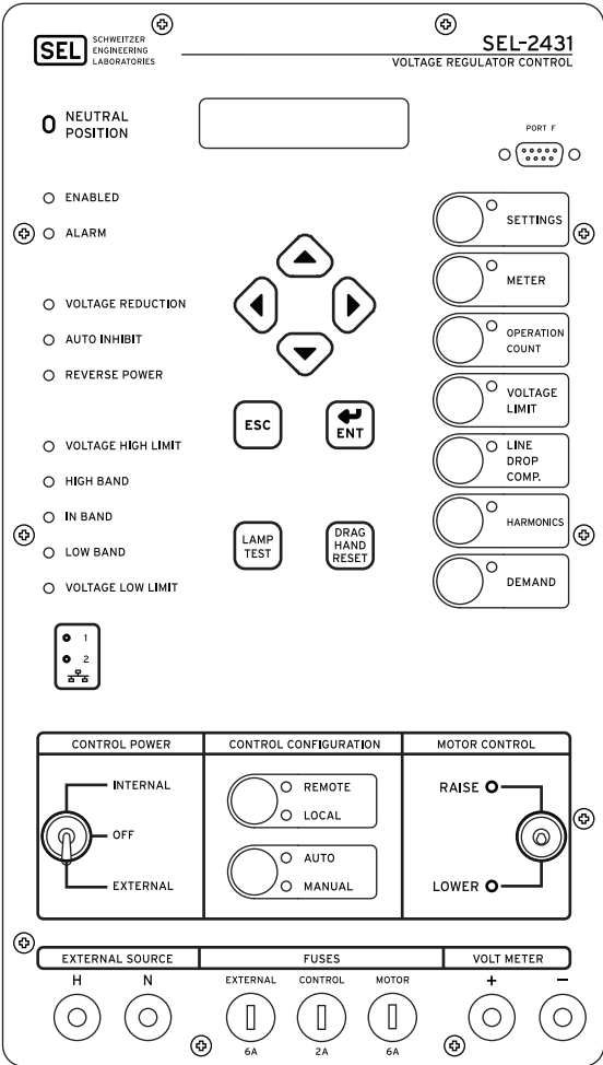
Front Panel With Raise/Lower Toggle Switch Option
