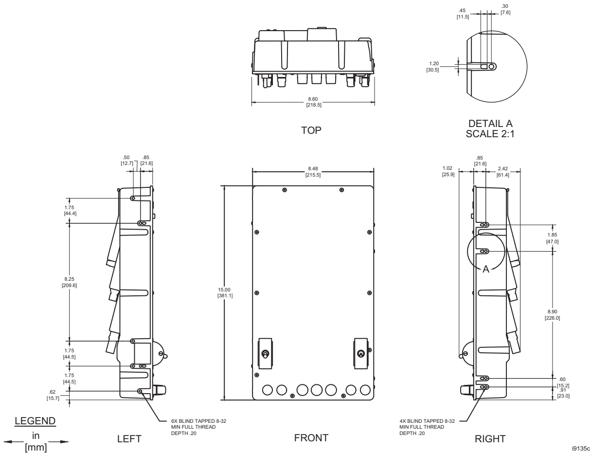
Figure 19 SEL-2431 Dimensions
