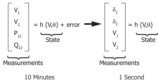
Figure 10 Synchrophasor Measurements Turn State Estimation Into State Measurement
