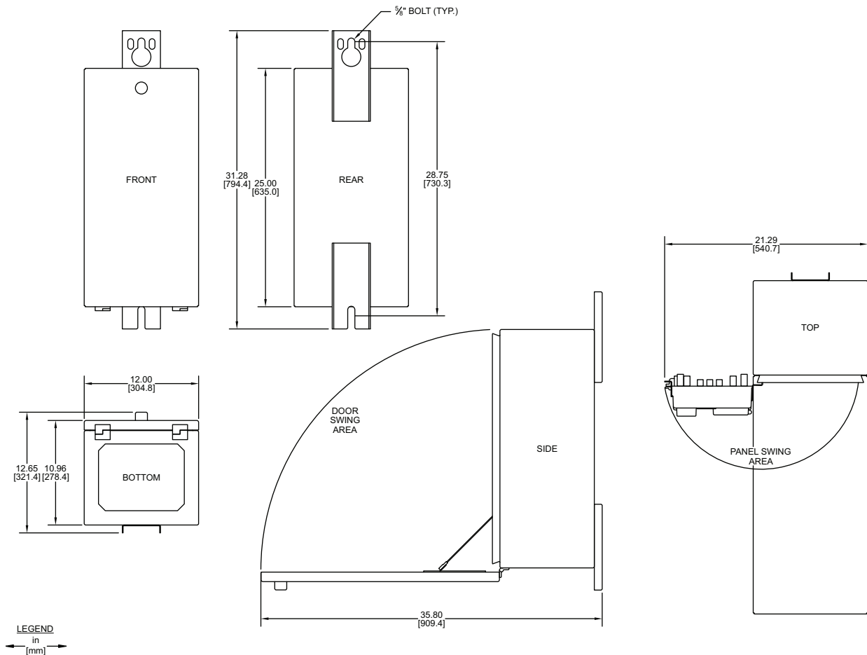
Figure 20 SEL-2431 Enclosure Dimensions
