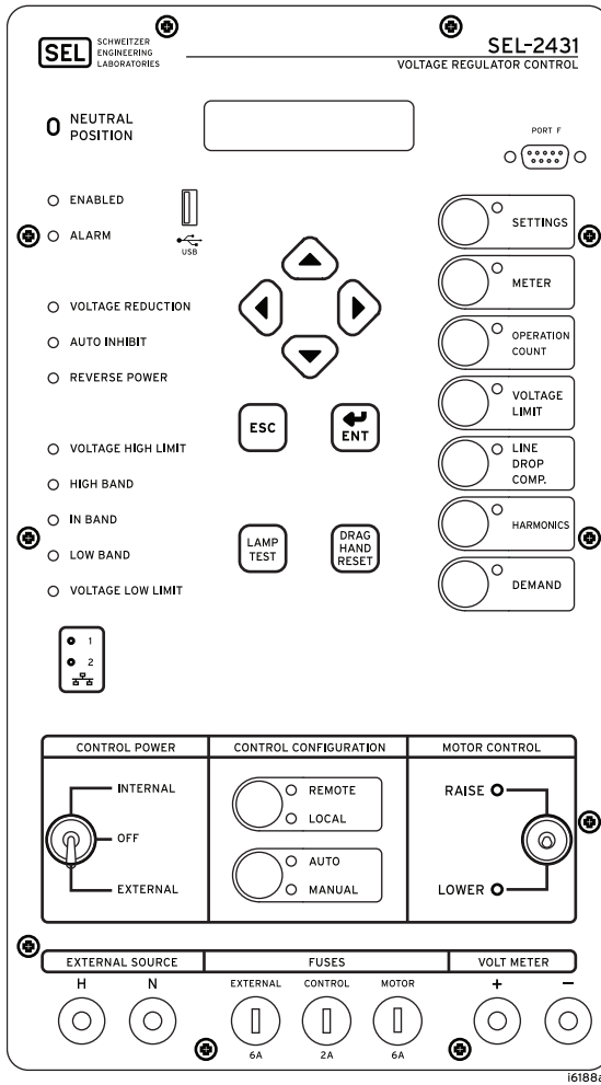
Front Panel With Raise/Lower Toggle Switch Option
