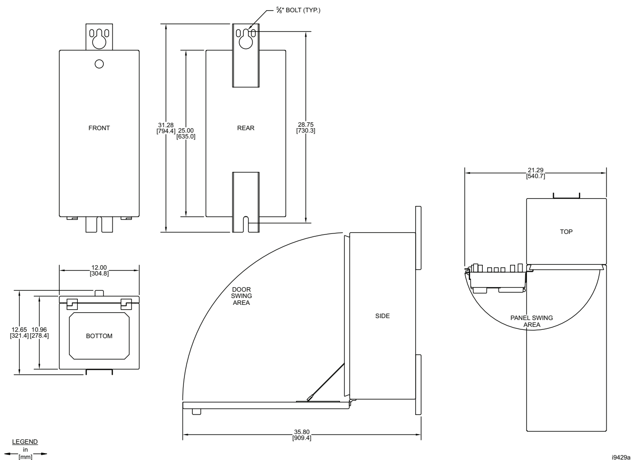
Figure 20 SEL-2431 Enclosure Dimensions
