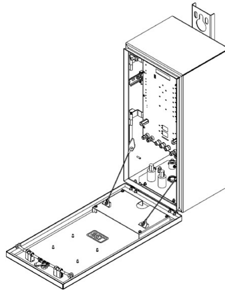
Figure 5 SEL-2431 Enclosure
