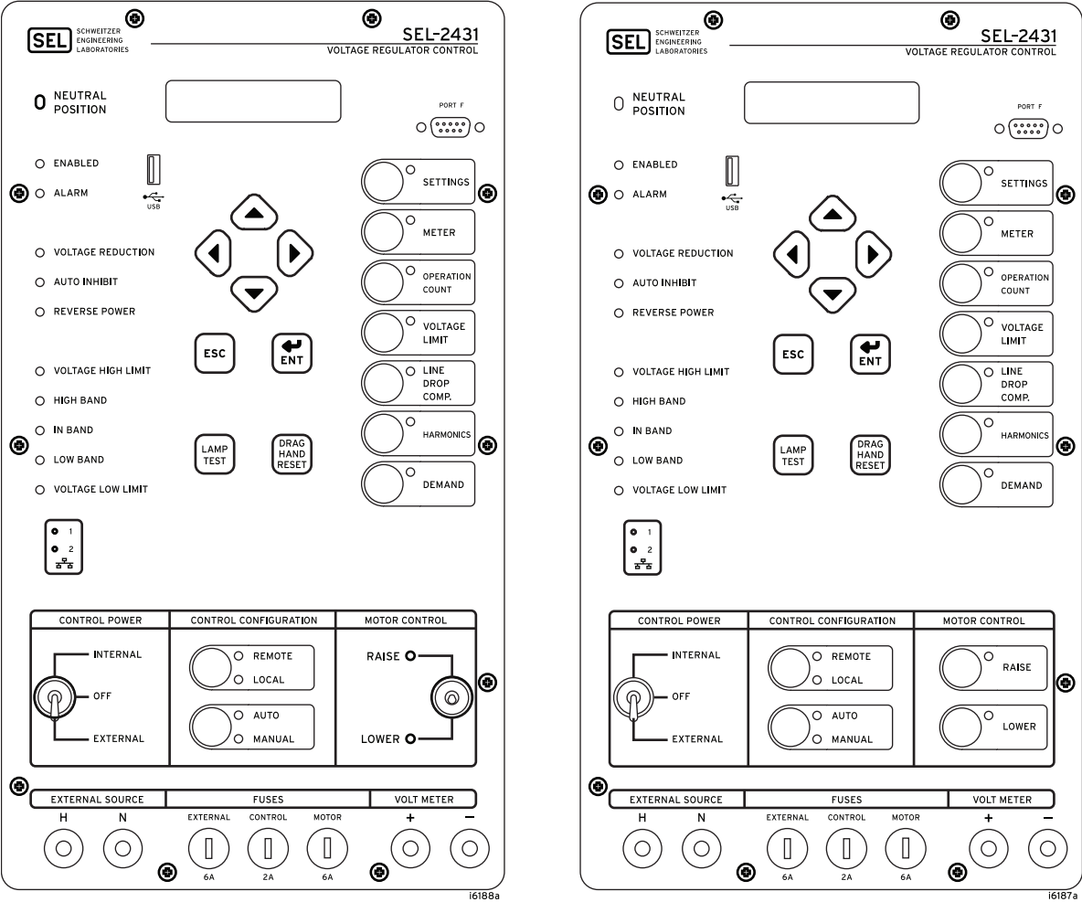
Figure 17 SEL-2431 Front Panels
