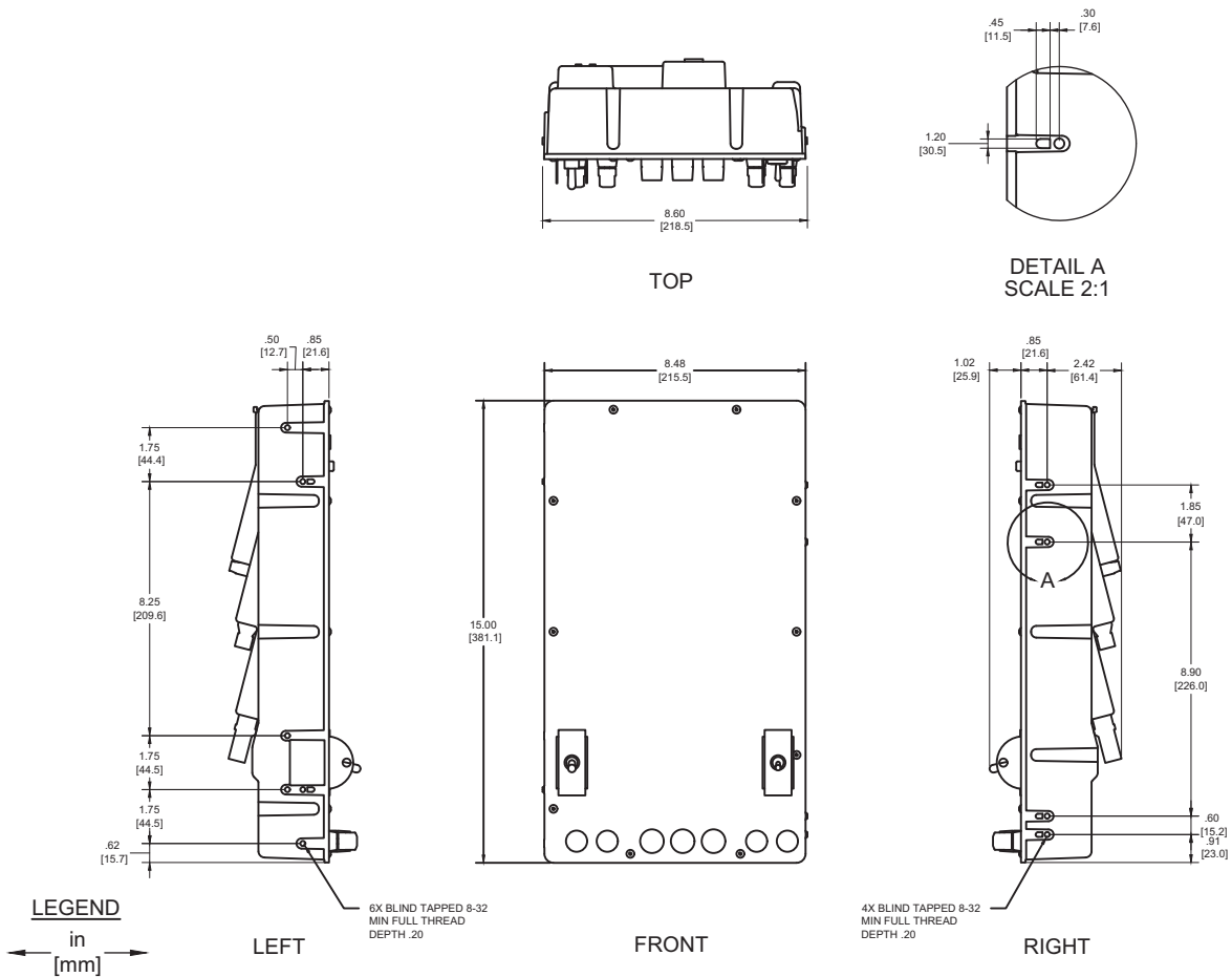
Figure 19 SEL-2431 Dimensions
