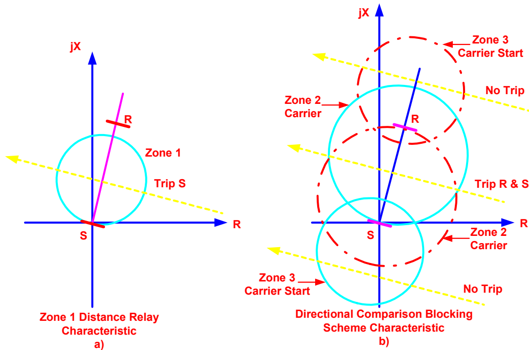
Figure 11 Zone 1 and Directional Comparison Blocking Scheme Characteristics
