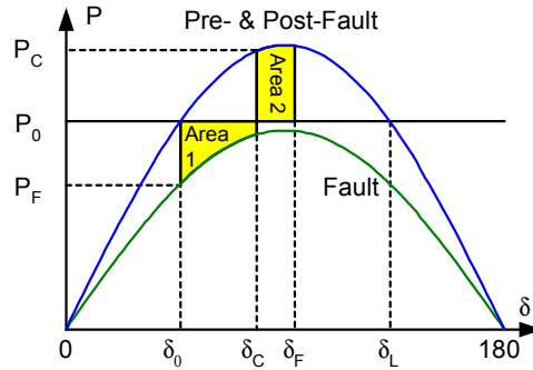
Figure 7 A Transiently Stable System
