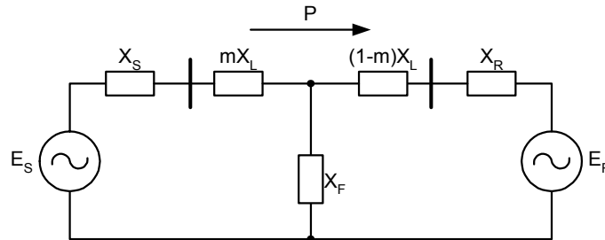
Figure 3 Two-source System With a Fault at Location m
