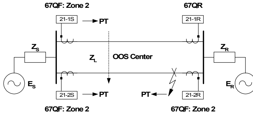
Figure 17 Use POTT Scheme to Gain Protection Security During System OOS
