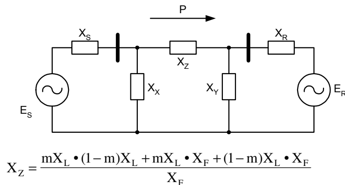
Figure 5 Delta-Wye Equivalent of the Faulted System
