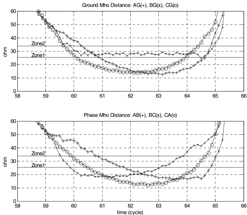
Figure 18 Distance Calculations for a BG Fault During System OOS
