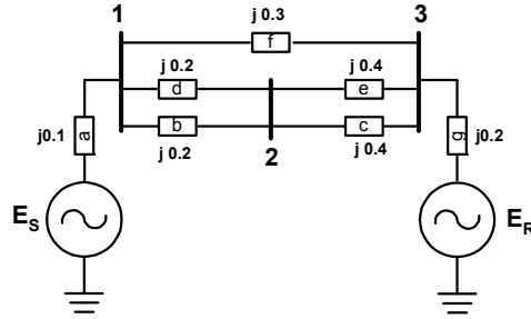
Figure A3 Example Network for Swing Locus Study
