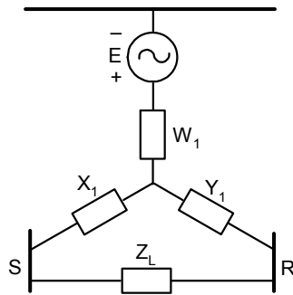
Figure A2 Wye-System Equivalent With Line Reintroduced Between Buses S and R
