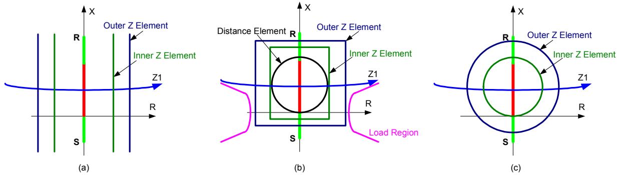
Figure 12 Different Double Blender OSB Characteristics
