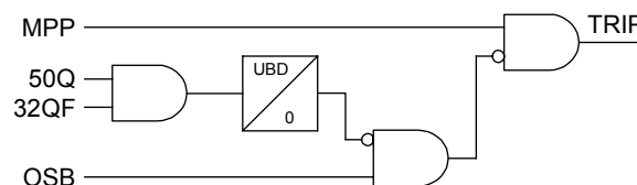
Figure 13 Distance Elements With OOS Block and Time Delayed 50Q Reset
