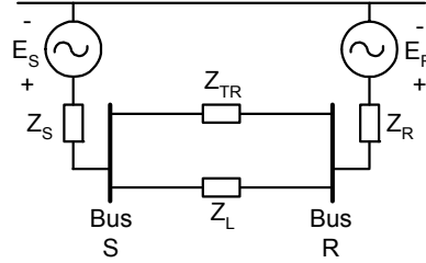
Figure A1 Two-Source System Equivalent
