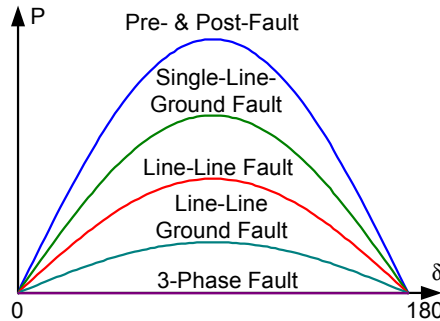
Figure 6 Power Transmission Capability of the Normal System and With Different Types of Faults
