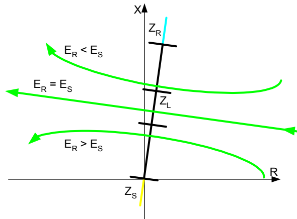
Figure 15 The Location of OOS Center Is a Function of Source Voltage Magnitudes
