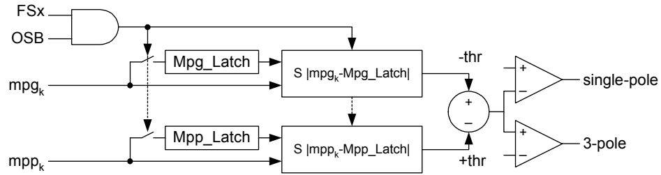
Figure 19 Fault Phase Selection Logic during System OOS
