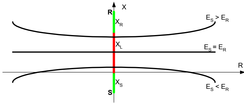
Figure 10 Z1 Trajectory of OOS for Different E_S and E_R Ratios
