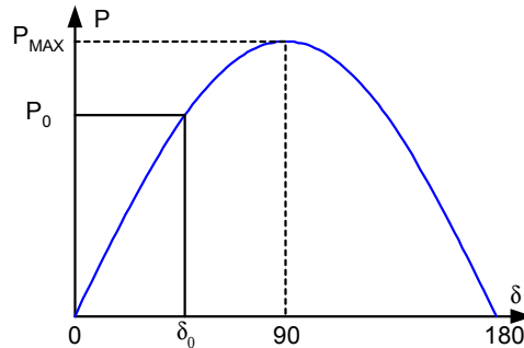
Figure 2 The Power Angle Curve
