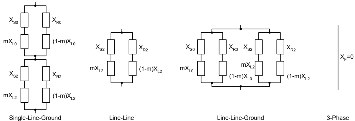
Figure 4 X_F for Different Types of Faults
