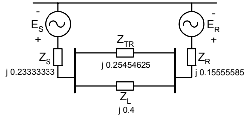
Figure A4 Equivalent Network Between Buses 2 & 3
