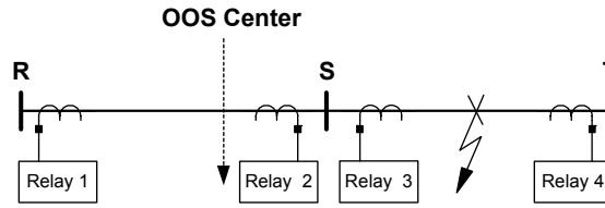
Figure 14 Use UBD to Coordinate With External Faults During OOS
