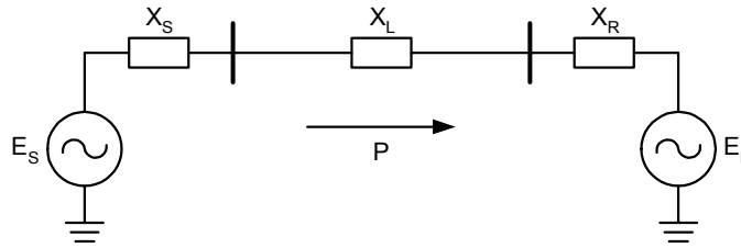
Figure 1 A Two-Source System
