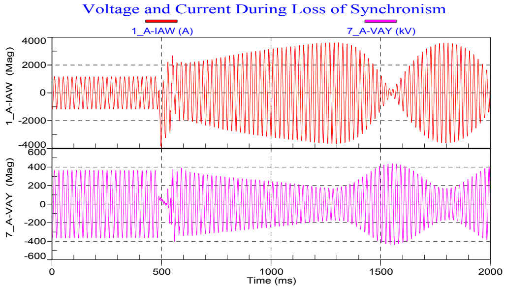
Figure 9 Voltage and Current During Loss of Synchronism
