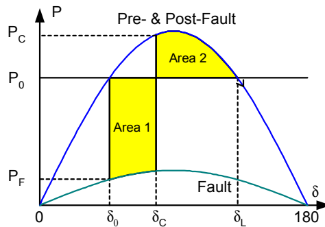
Figure 8 A Transiently Unstable System
