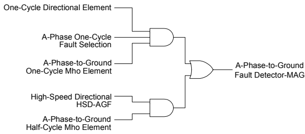
Figure 2. A-Phase Impedance Loop Half- and One-Cycle Combination Logic
