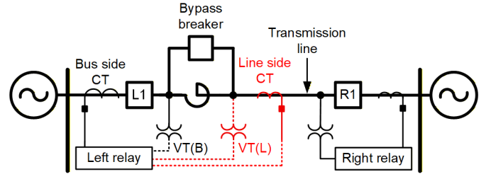
Fig. 2 CT and VT connection options
