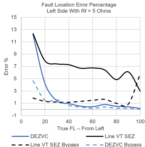
Fig. 15 Fault location error for the left relay ( R = 5 ohms)
