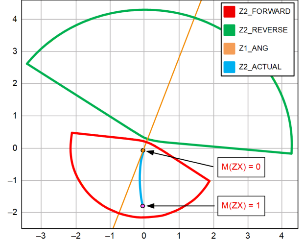
Fig. 14 Z2 impedance for reactor faults with line VTs for sample system
