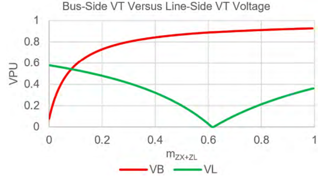
Fig. 6 VT(B) and VT(L) voltages
