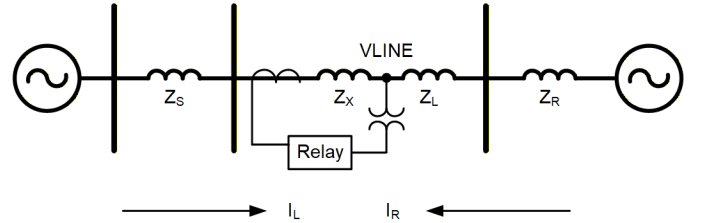
Fig. 18 System diagram
