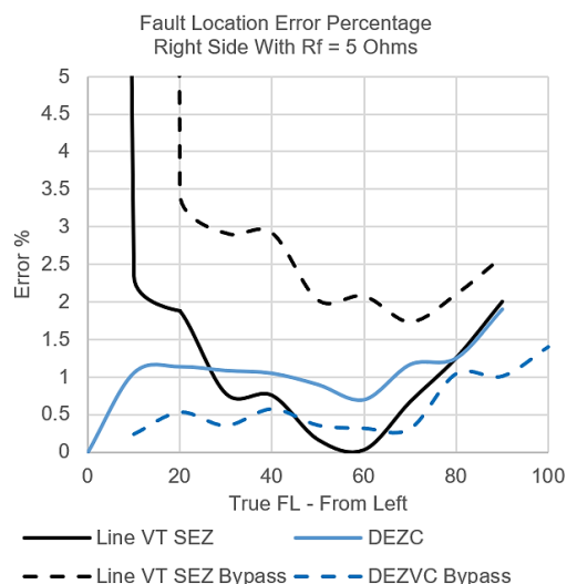
Fig. 16 Fault location error for the right relay ( R = 5 ohms)
