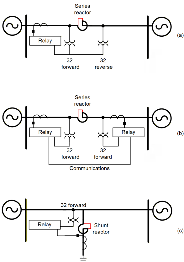
Fig. 19 Series reactor versus shunt reactor
