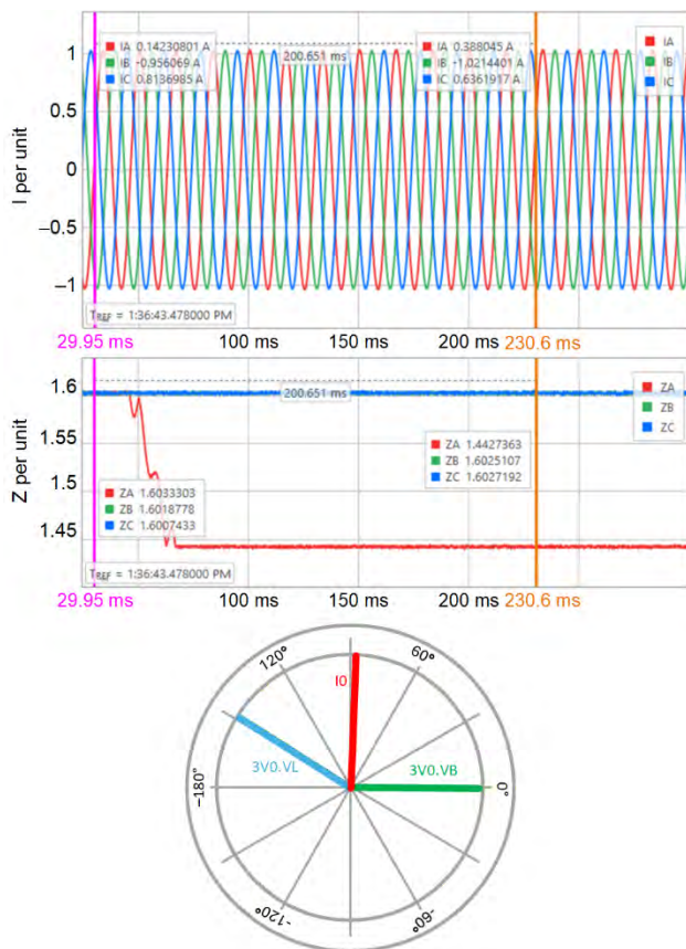
Fig. 20 10 percent turns shorted in series reactor
