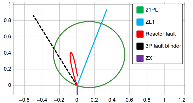
Fig. 9 21PL apparent impedance trajectory for bolted three-phase reactor faults
