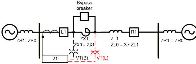
Fig. 4 Sample system
