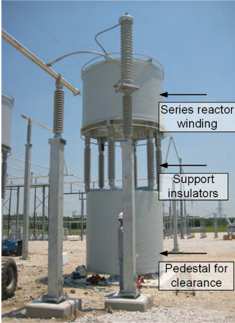
Fig. 1 Air-core series reactor installed at 138 kV substation
