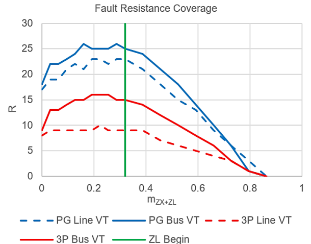
Fig. 13 Fault resistance coverage for Oncor example line
