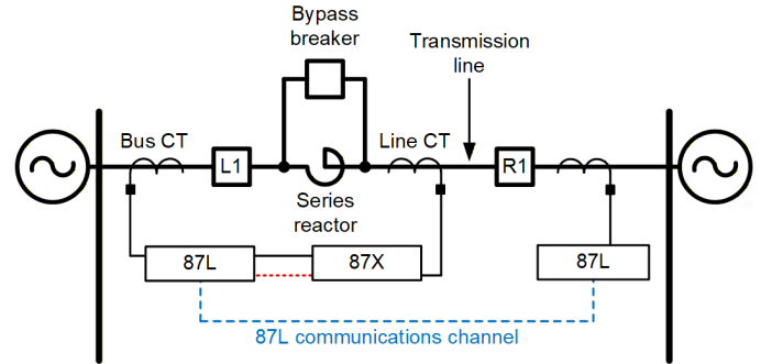
Fig. 3 Preferred 87X and 87L configuration
