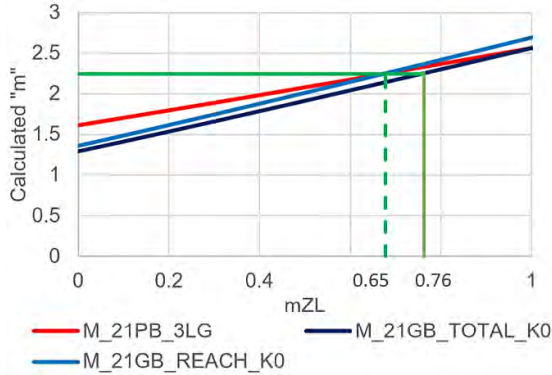
Fig. 11. Mho distance “m” calculation
