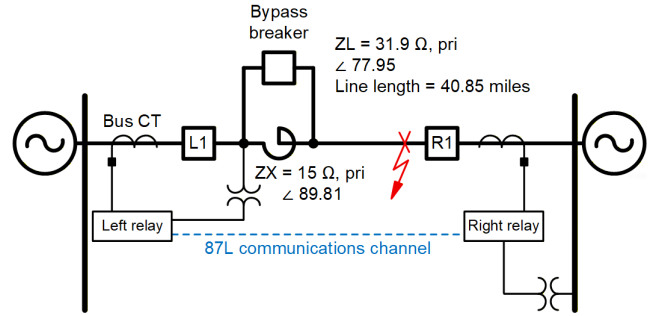
Fig. 12 Test system
