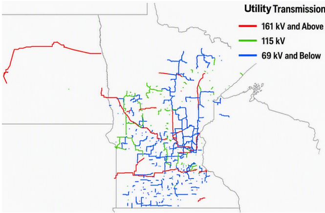
Fig. 2. Map of the utility transmission and subtransmission systems.
