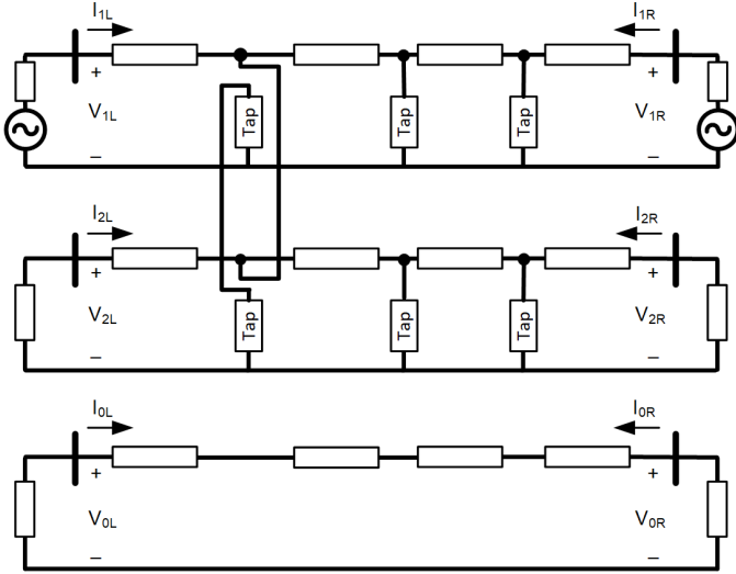
Fig. 4. Sequence network (with floating zero-sequence network) for the system in Fig. 1 for a broken conductor event in one of the tap circuits.
