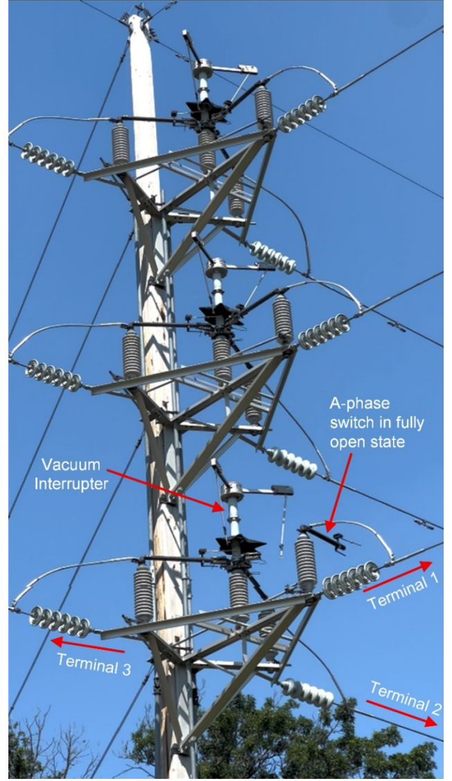
Fig. 8. A-phase switch in fully open state isolating Terminal 1 from the line.
