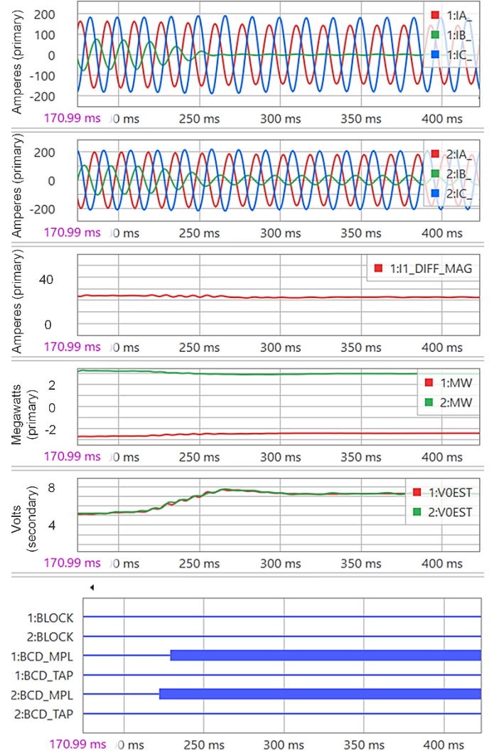
Fig. 11. Currents, megawatts, estimated remote-end zero-sequence voltage and blocking signal for the broken conductor event between the relay terminal and the first tap.
