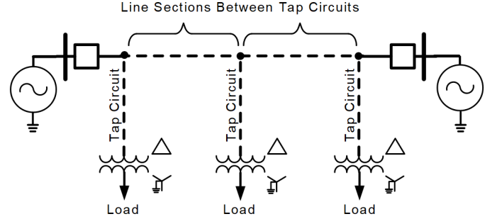
Fig. 1. Example of a tapped transmission line showing sections where traditional BCD schemes lack dependability (dashed lines).
