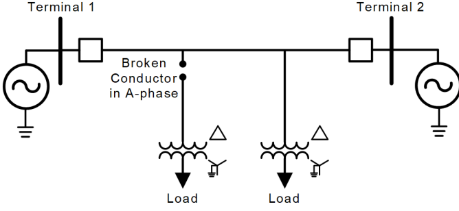
Fig. 14. Single-line diagram of a 115 kV transmission line with a broken conductor on the tap circuit in A-phase.
