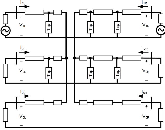
Fig. 3. Sequence network of the system in Fig. 1 for a broken conductor event between adjacent tap connections.
