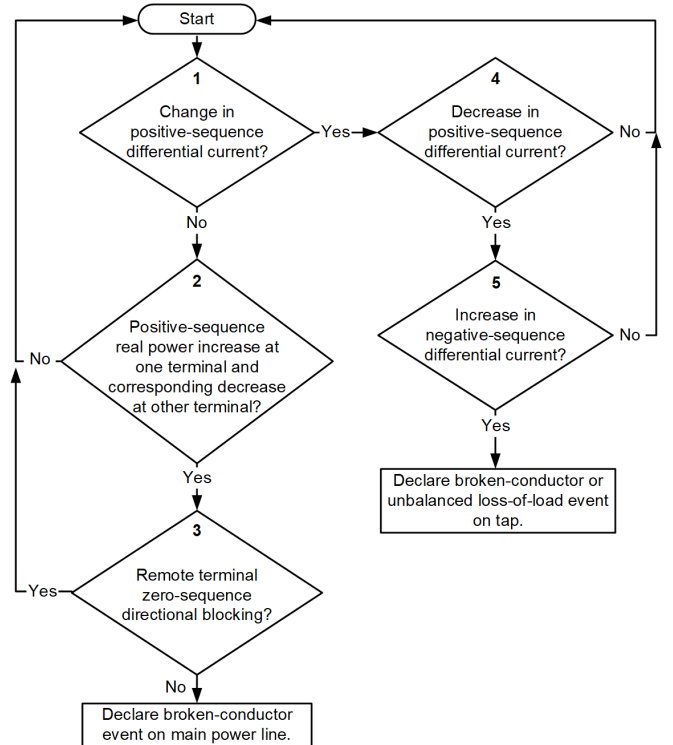
Fig. 5. Flowchart of the proposed BCD algorithm conditions for a two-terminal tapped transmission line.
