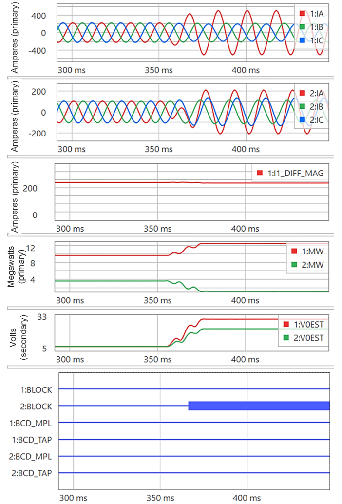
Fig. 13. Currents, megawatt (MW), estimated remote-end zero-sequence voltage, and blocking signal at Terminals 1 and 2 for the broken conductor event outside the protected line section.
