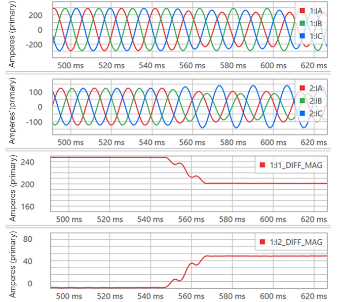
Fig. 15. Currents at Terminals 1 and 2 for the broken conductor event on a tap circuit, shown in Fig. 14.
