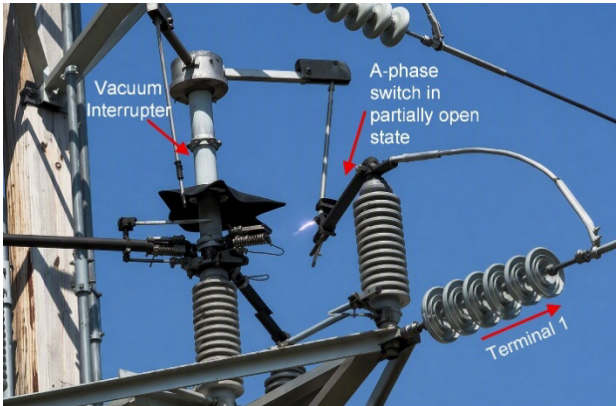
Fig. 7. Short duration arcing during operation of the A-phase switch.
