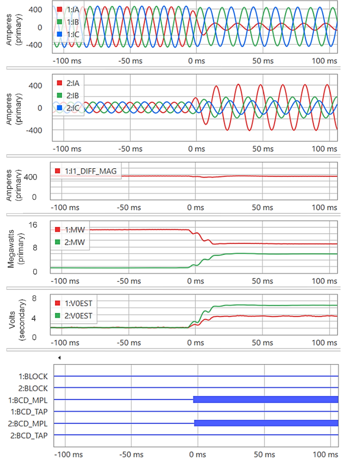
Fig. 9 Currents, megawatts, estimated remote-end zero-sequence voltage, and blocking signals at Terminals 1 and 2 for the broken conductor event between tap locations.
