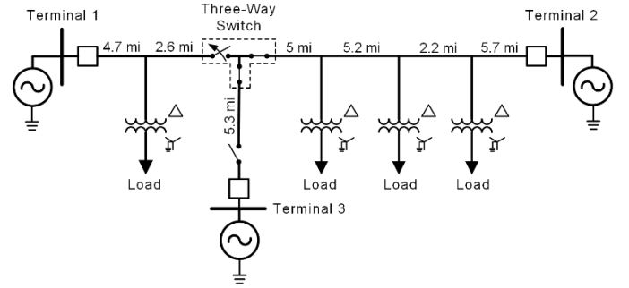
Fig. 6. Single-line diagram of the 69 kV transmission line under test.
