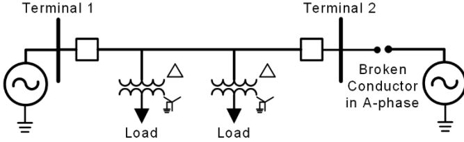
Fig. 12. Single-line diagram of a 115 kV transmission line with an out-of-zone broken conductor in A-phase.
