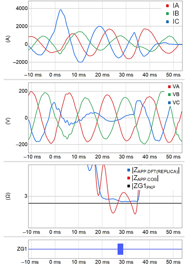
Fig. 19. Field event from IBR with m using fault loop polarization.
