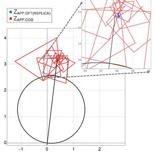
Fig. 16. Apparent impedance calculations for the fault in Fig. 15.
