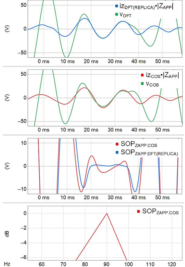
Fig. 20. Field event from IBR with m using fault loop polarization.
