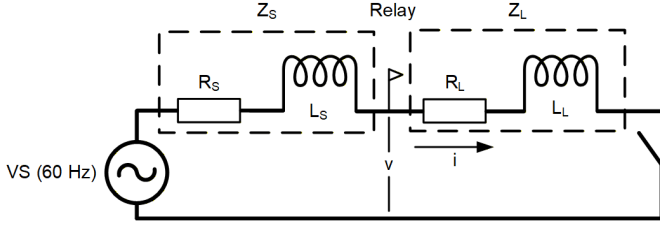
Fig. 4. Simple system with a 60 Hz source.
