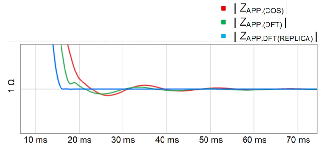
Fig. 6. Apparent impedance calculations of filtering techniques with dc content in the signal.
