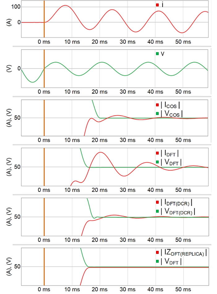
Fig. 5. Digital filter outputs when applying signals v and i .
