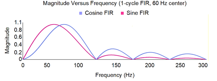
Fig. 10. FIR filter signal attenuation to interharmonic frequencies.
