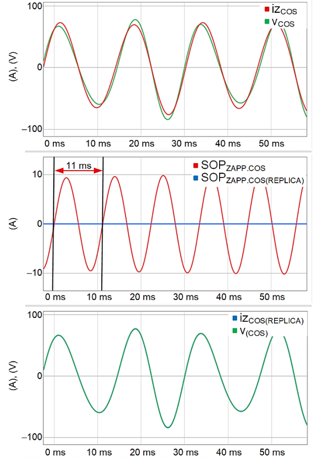
Fig. 14. Comparison of using replica current filter versus not.
