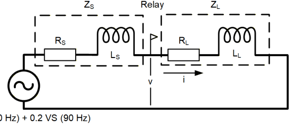
Fig. 11. Circuit with a 60 Hz and 90 Hz voltage source.
