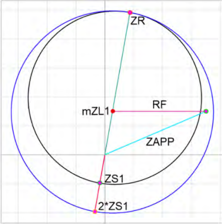
Fig. 2. Characteristics for Relay 1: black n = 1 and blue n = 2 ; characteristic for Relay 2: black only.
