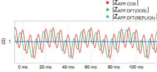
Fig. 13. Apparent impedance calculations of filtering techniques with 90 Hz content in the signal.
