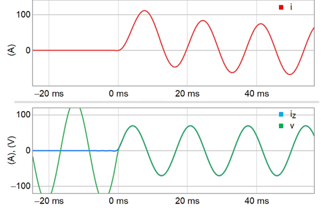
Fig. 8. i_z relationship with v .
