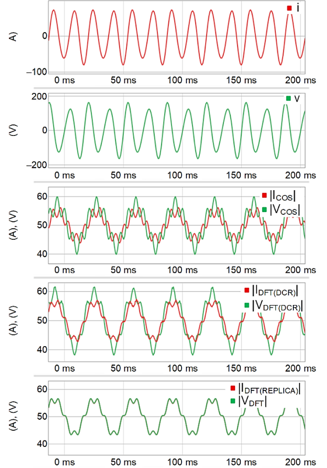
Fig. 12. Filter response to a 90 Hz signal.
