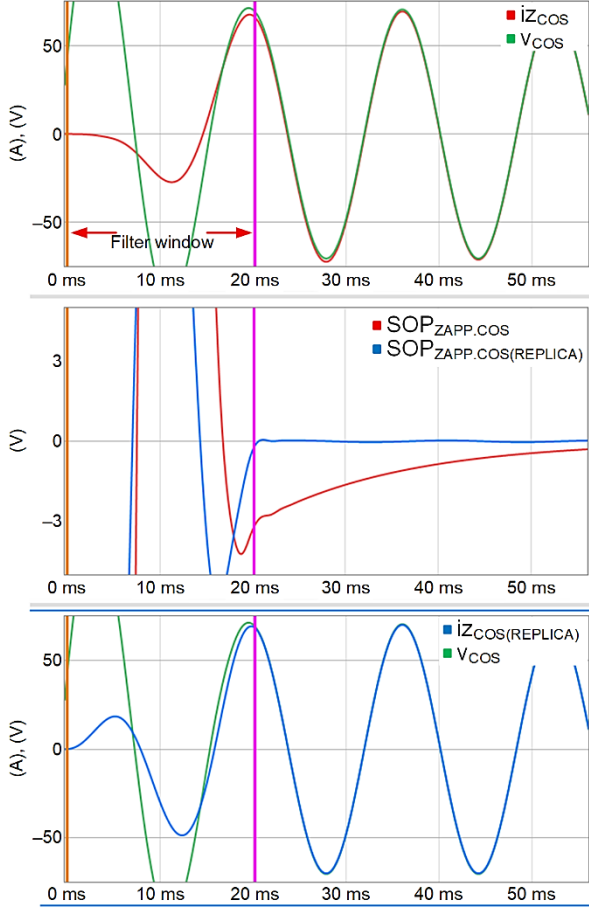
Fig. 9. Comparison of using a replica current filter versus not using a replica current filter.
