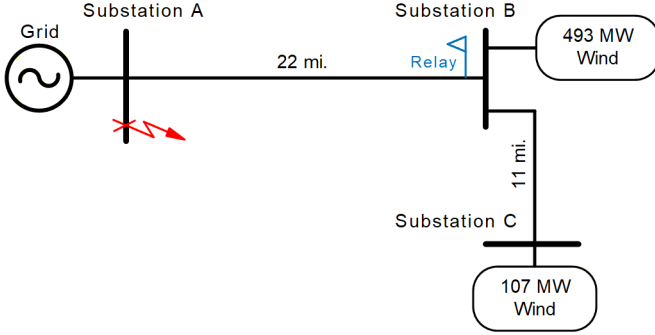
Fig. 18. Transmission system from field event.
