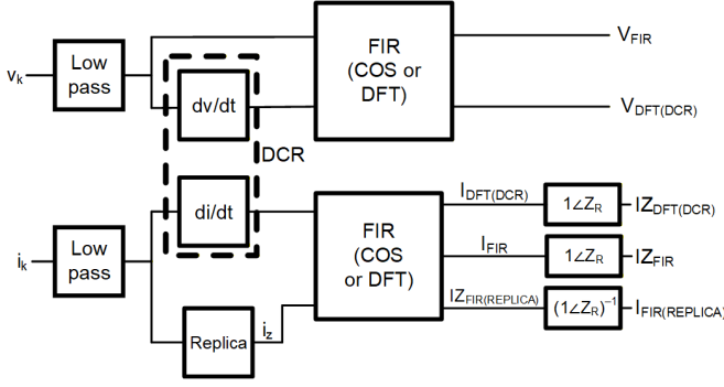
Fig. 7. Simplified filtering diagram.
