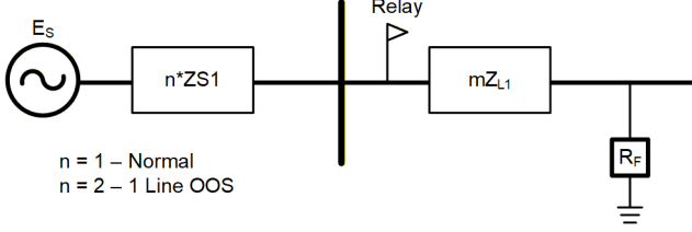
Fig. 1. Radial system with a fault located at mZ_{L1} .
