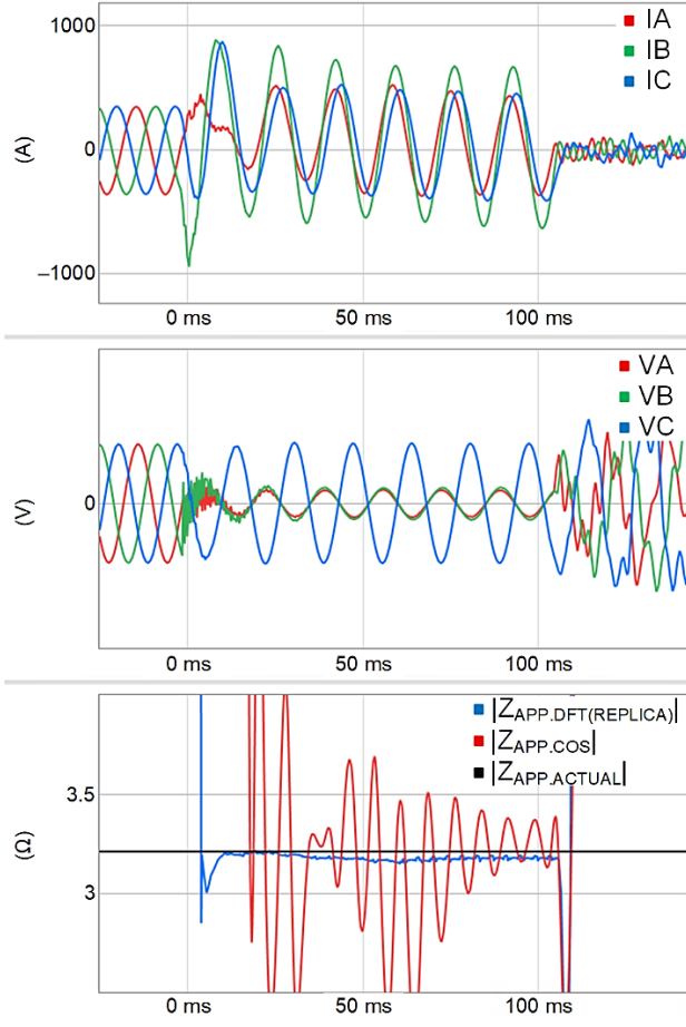
Fig. 15. |Z_{APP}| for an ABG fault from an IBR model simulation.
