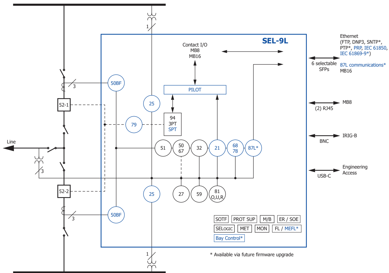
Figure 3 Feature Overview
