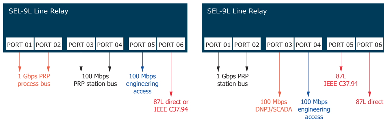
Figure 10 Network Configuration Examples
