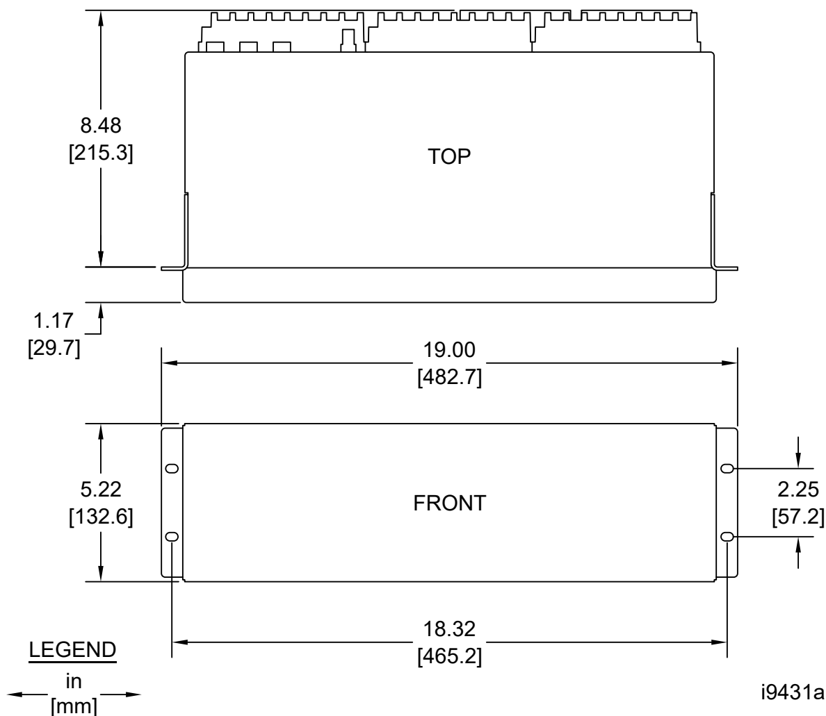
Figure 15 SEL-9L Rack-Mount Dimensions (All Models)
