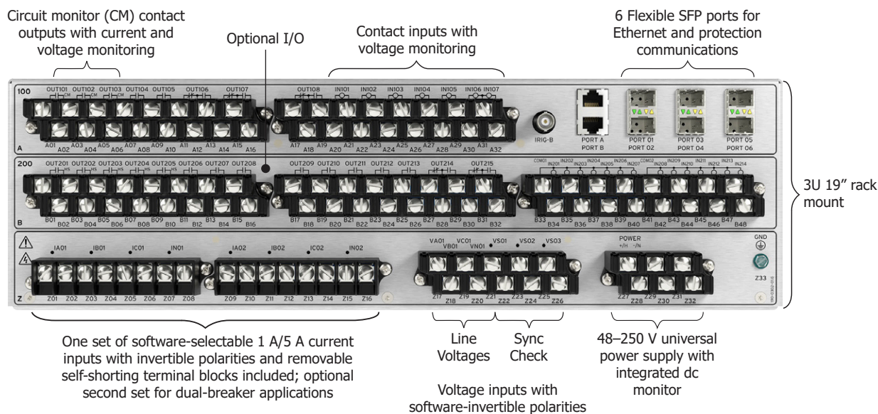
Figure 2 Rear Panel
