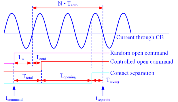
Fig. 3 A reproduction of Fig. 1 in [4]. Controlled opening sequence.
