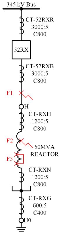
Fig. 2 Ameren reactor installation. Only one set of redundant CTs is shown at each location to reduce clutter.
