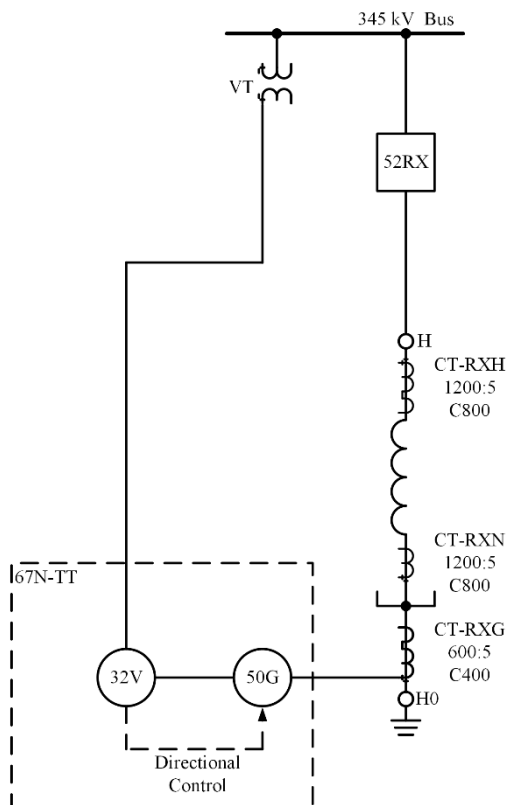
Fig. 7 67N turn-to-turn fault scheme.
