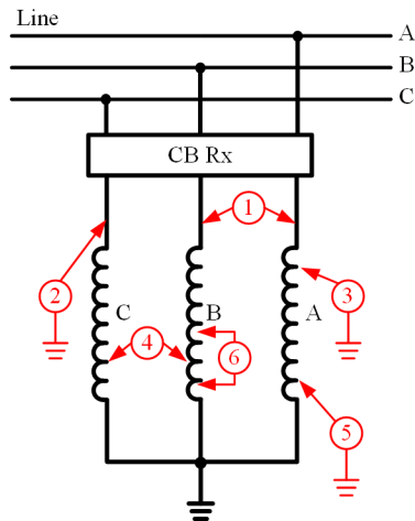
Fig. 4 A reproduction of Fig. 2 in [1]. Types of faults in a shunt reactor.
