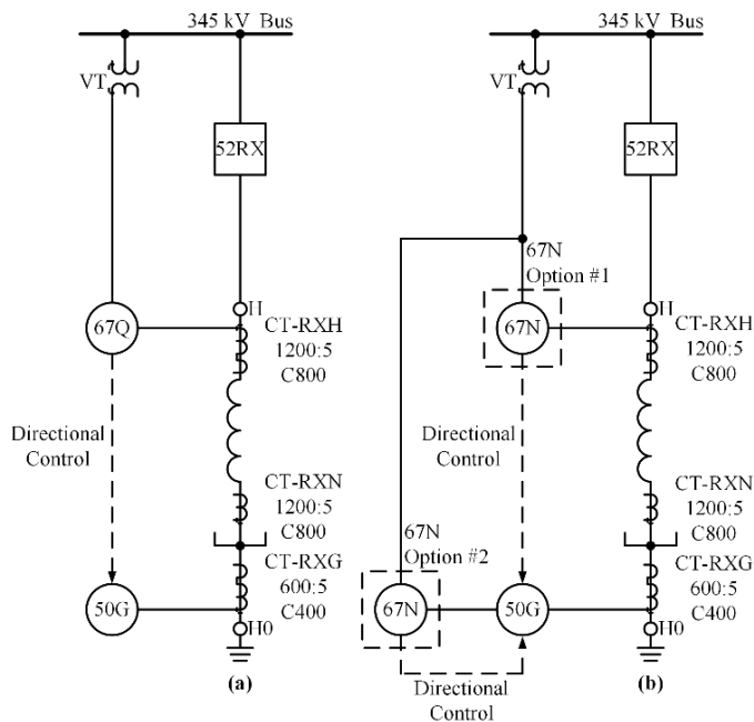
Fig. 6 (a) Turn-to-turn fault protection for grounded reactor using negative-sequence directional control; (b) turn-to-turn fault protection for grounded reactor using zero-sequence directional control.
