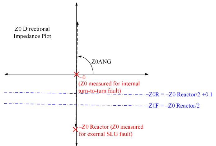
Fig. 9 Simplified Z0 directional impedance plot showing the approximate apparent impedance for an internal turn-to-turn fault and an external SLG fault.
