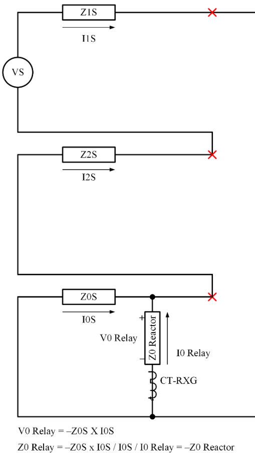
Fig. 8 External SLG fault sequence diagram.
