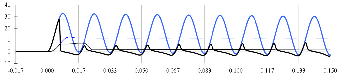
Fig. 10 Simulated CT response of the CT-RXG for an external fault.
