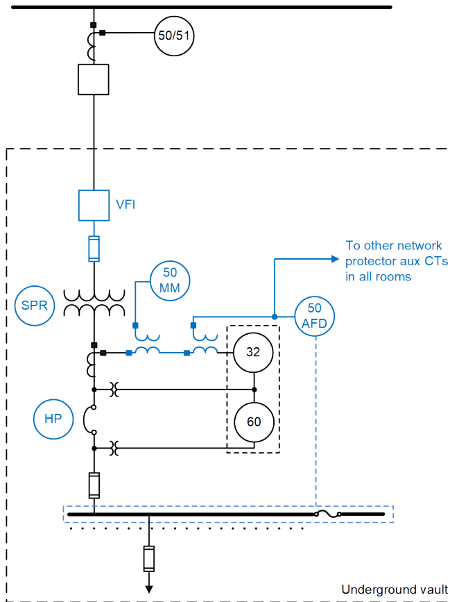
Fig. 13. Upgraded protection standard for 480 V vaults.
