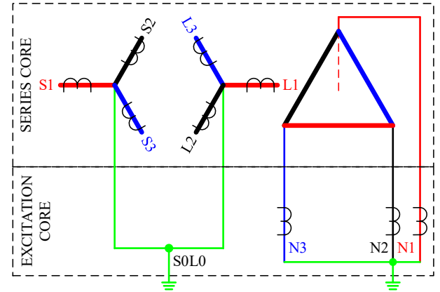
Fig. 23. Secondary winding ATB differential element, 87S
