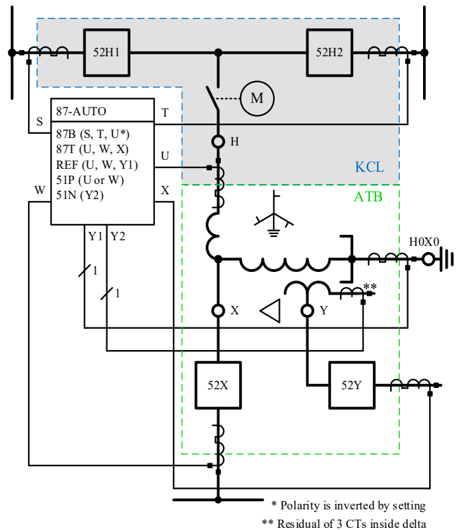
Fig. 11. Transformer dual-breaker application with recommended protection
