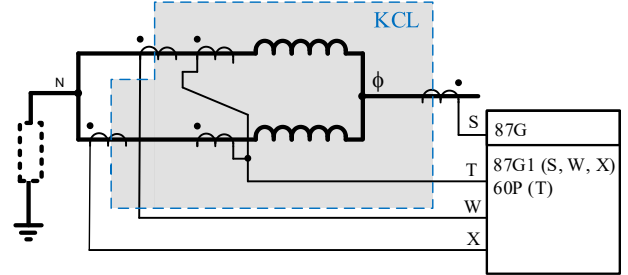
Fig. 18. Generator and split-phase (60P)
