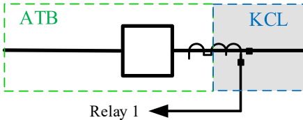
Fig. 6. Zones of protection with a single CT at the zone boundary
