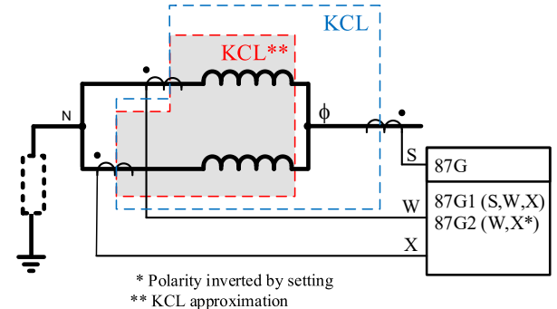
Fig. 19. Generator and split-phase (87)
