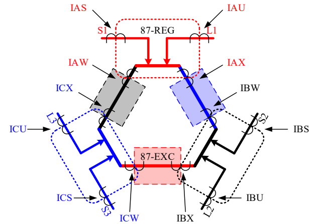
Fig. 24. Single-core KCL differential, 87-REG and 87-EXC
