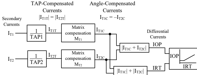
Fig. 4. Simplified ATB-based current differential protection
