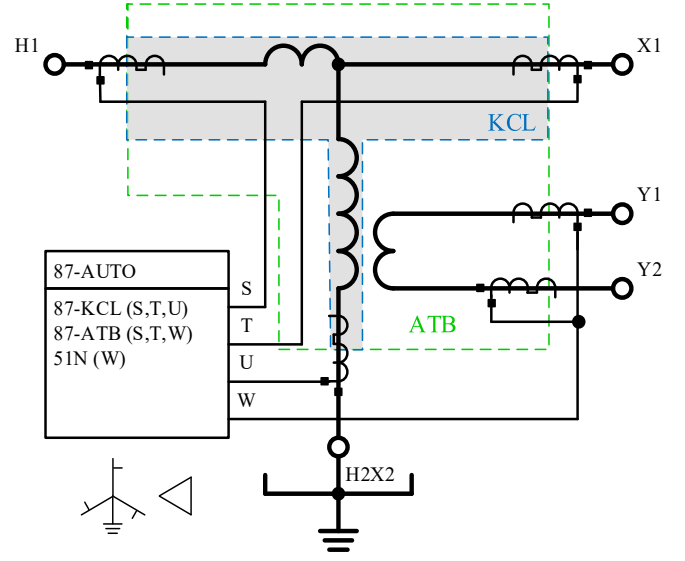
Fig. 12. Bank of single-phase autotransformers with recommended protection
