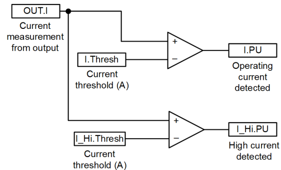
Fig. 9 Current Threshold Logic
