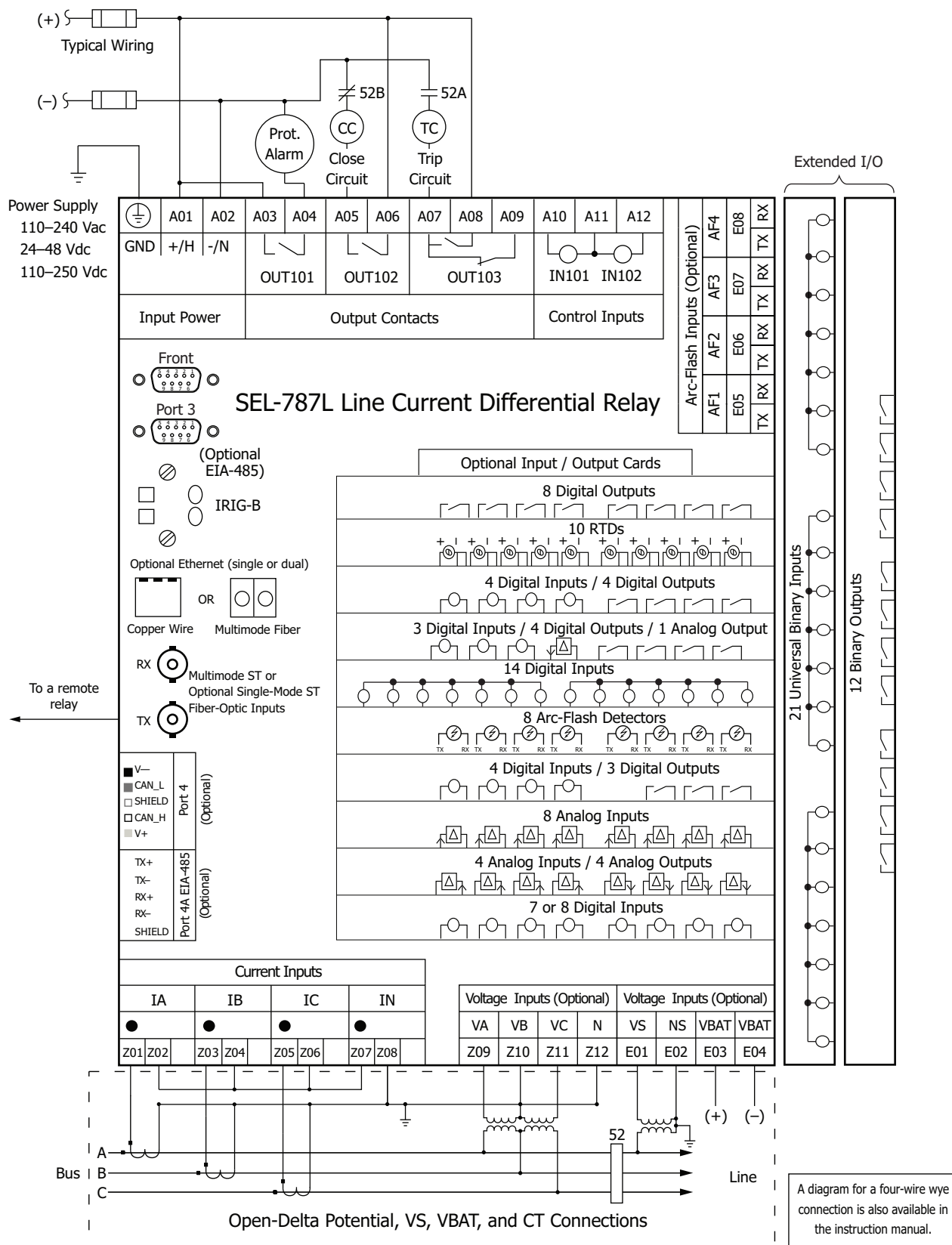
Figure 41 SEL-787L Hardware Overview
