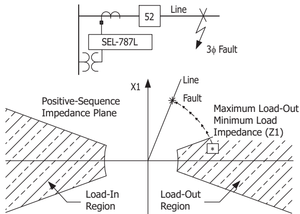
Figure 7 Load-Encroachment Characteristics
