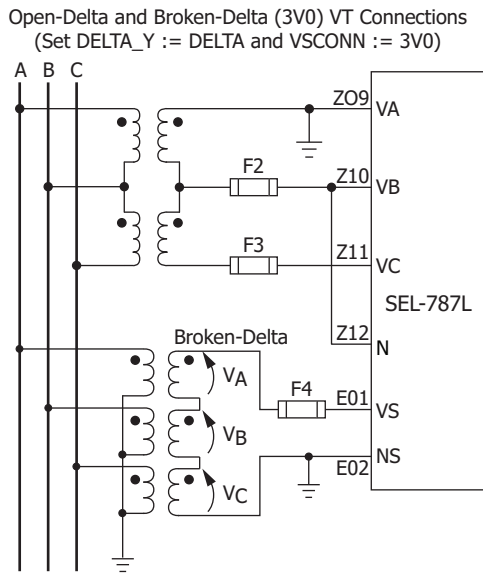
Figure 10 Broken-Delta Connections
