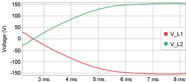
Fig. 9. 6 ms, 1 Msps voltage waveform
