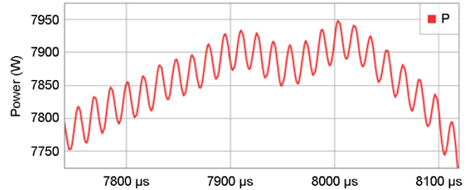
Fig. 13. Instantaneous power ripple
