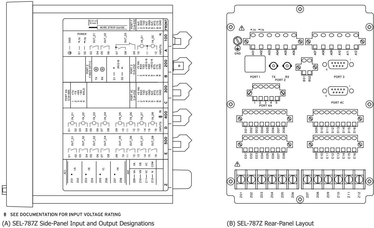
Figure 31 No Ethernet, EIA-232 Serial Communications, EIA-232/EIA-485 Communications Card, 8 DI Card, 8 DO Card (Form A), and SEL-HZM With HZM-Bypass Relay Option (Relay MOT 0787Z001AA03A2A8500010111)
