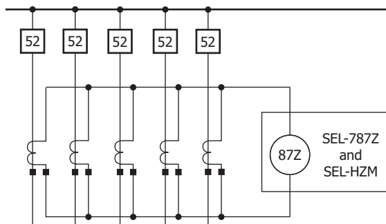
Figure 33 Example Bus Protection (One Phase Shown Connected)
