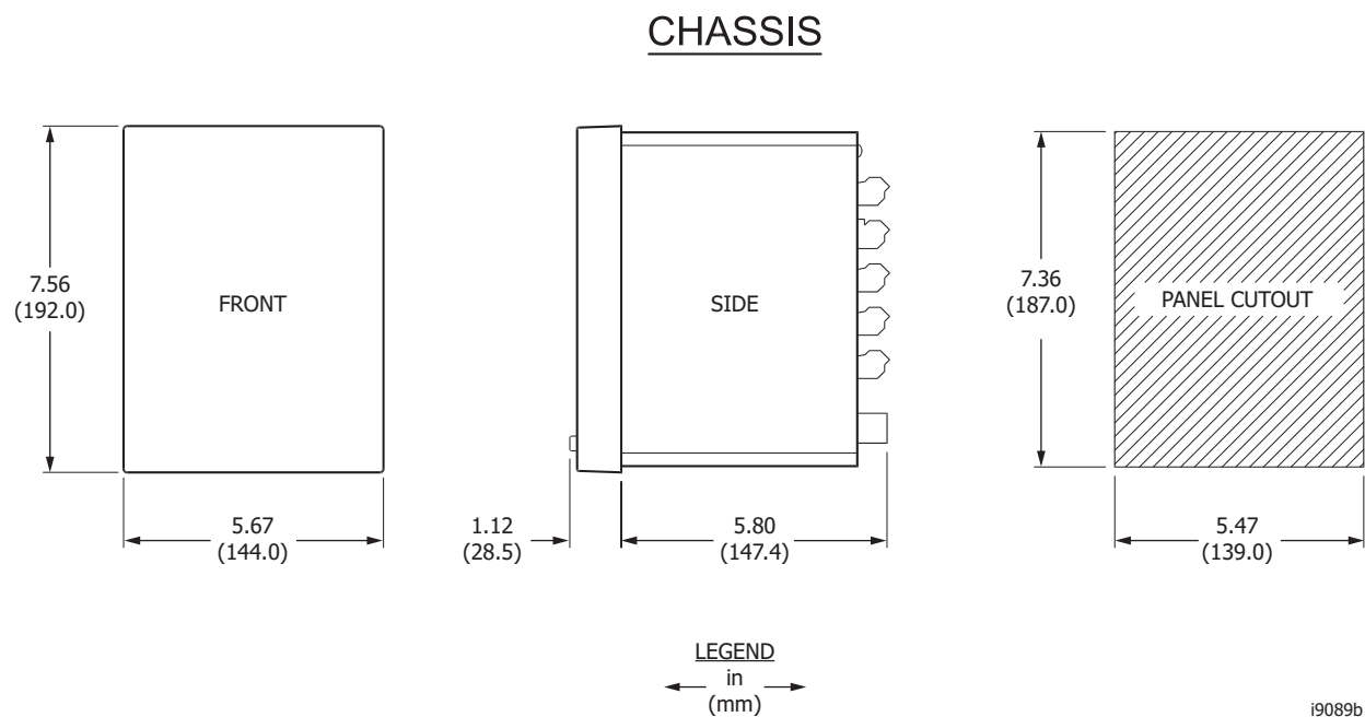
Figure 24 SEL-787Z Dimensions
