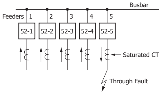
Figure 2 CT Saturation Resulting From a Through Fault
