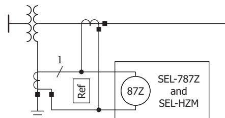
Figure 34 Transformer With Grounded-Wye Connected Winding
