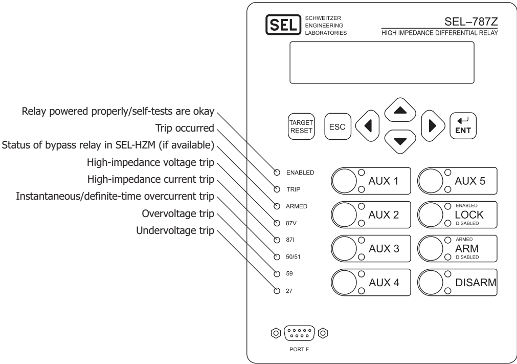
Figure 30 Front-Panel Overview
