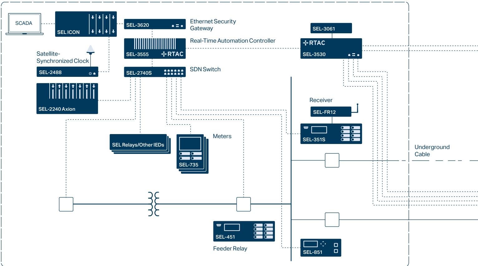
Substation
