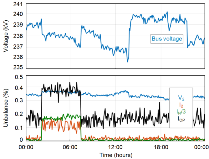
Fig. 33. Measured profile of several signals throughout one summer day.
