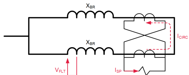
Fig. 19. Simplified circuit used to determine split-phase element pickup
