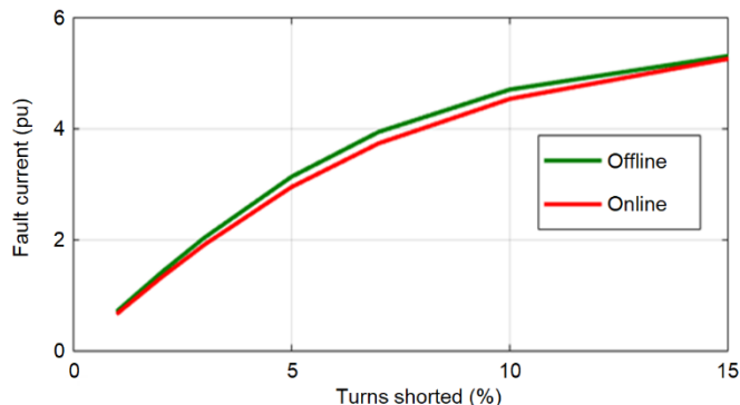
Fig. 21. Fault current levels for turn-to-turn faults
