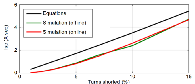
Fig. 20. Comparison of simplified split-phase equations with model response
