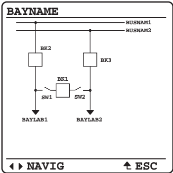
Figure 22 Breaker-and-a-Half
