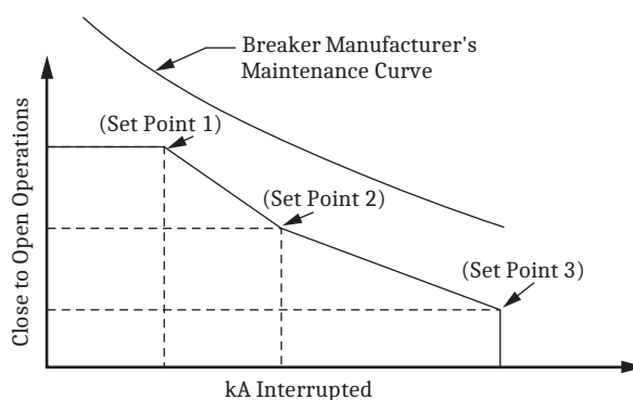
Figure 32 Breaker Contact Wear Curve and Settings
