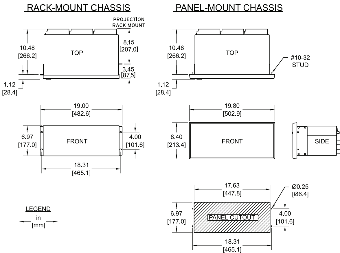
Figure 37 Dimensions for Rack- and Panel-Mount Models
