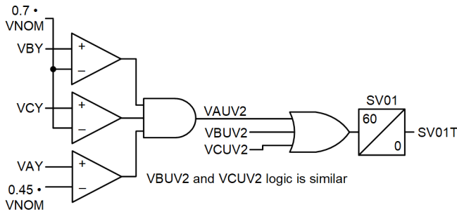
Fig. 7. VY Undervoltage Securing Logic for an Open-Phase Condition on the A-Phase
