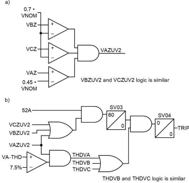
Fig. 9. (a) VZ Undervoltage Securing Logic for an Open-Phase Condition on the A-Phase (b) V-THD OPD Scheme
