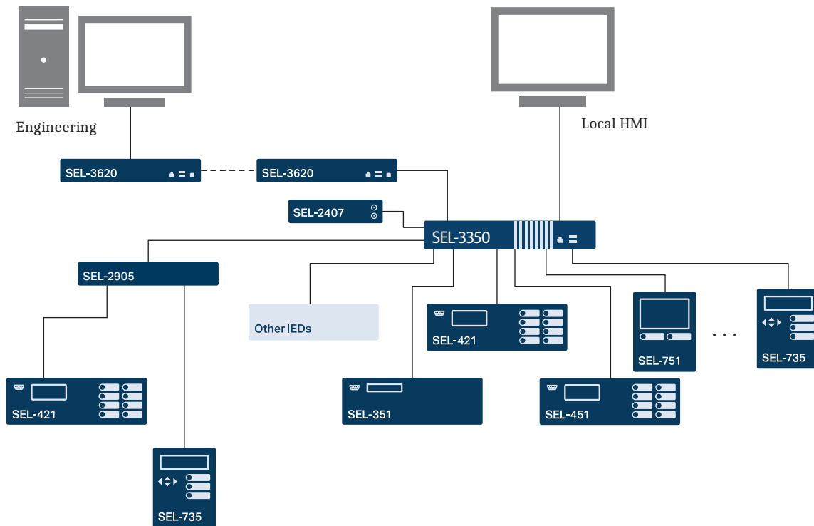
Figure 1 Engineering Communication Through a Serial Access Point
