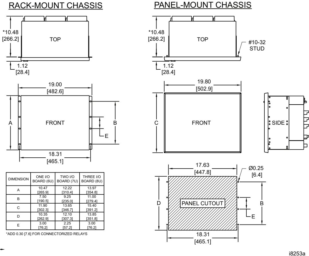
Figure 46 SEL-400G Dimensions for Rack- and Panel-Mount Models
