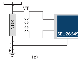
(c) Injecting current via broken-delta winding of NGT
