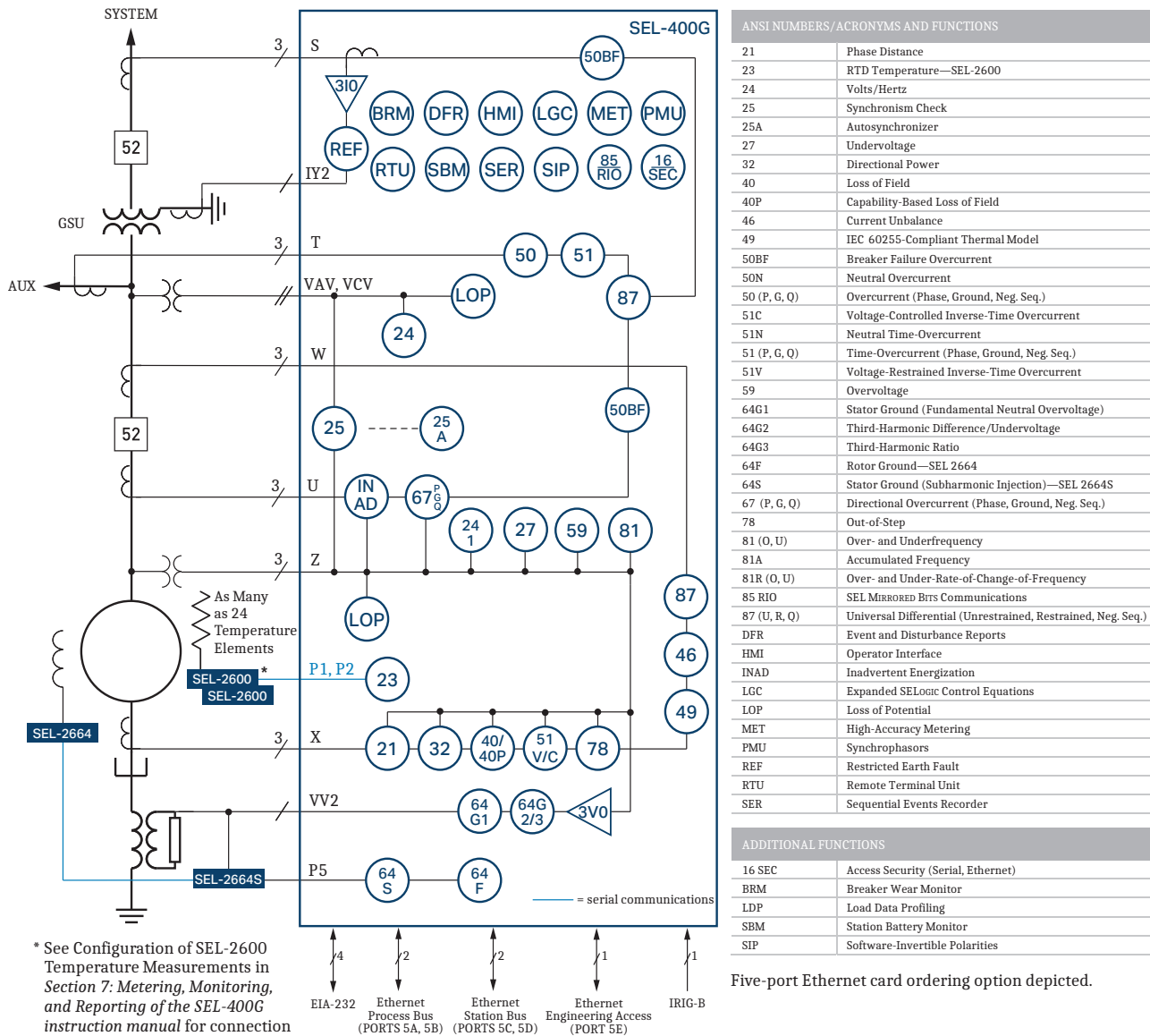
Figure 1 Functional Diagram
