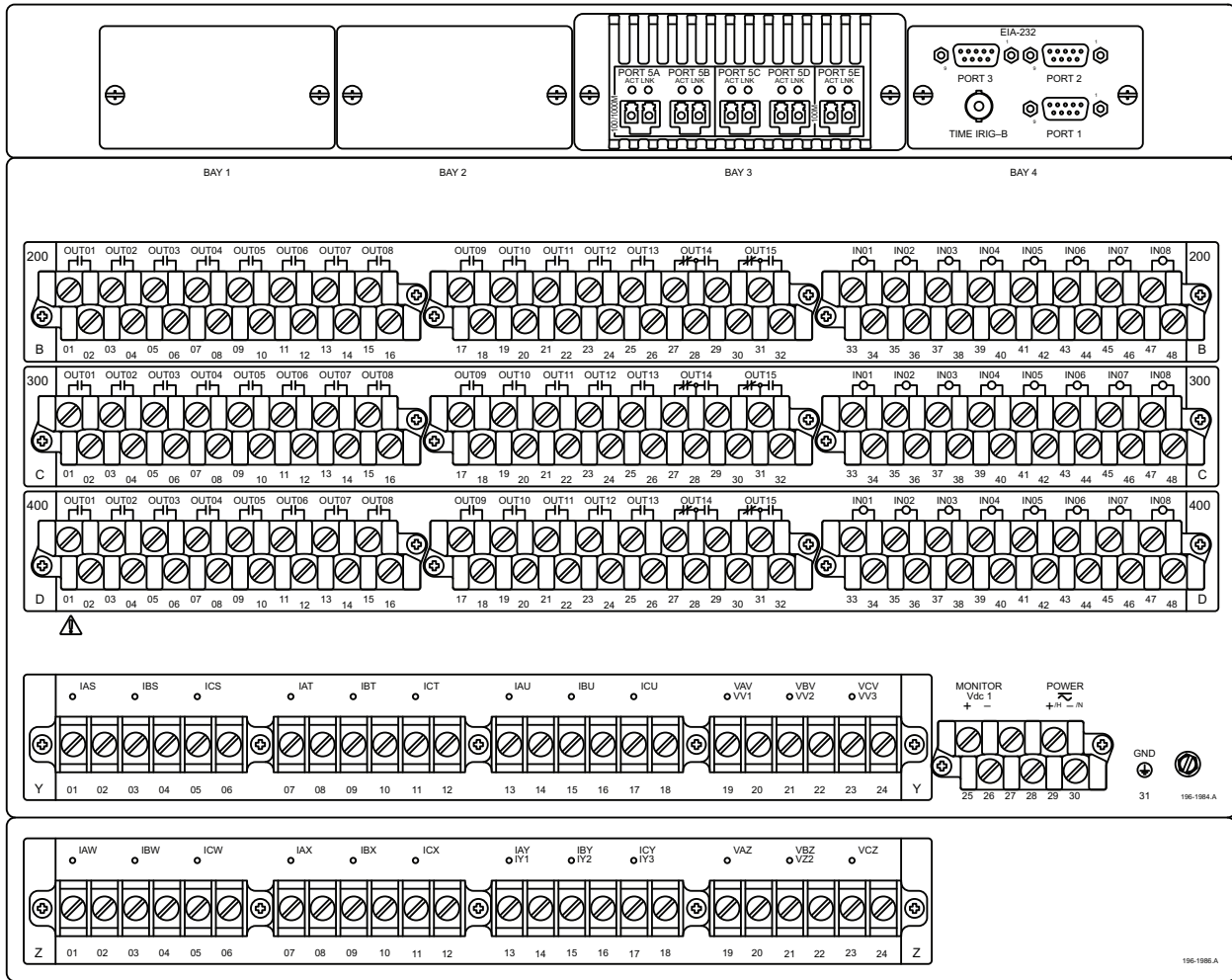
Figure 39 8U Rear-Panel Diagram With Fixed Terminal Blocks
