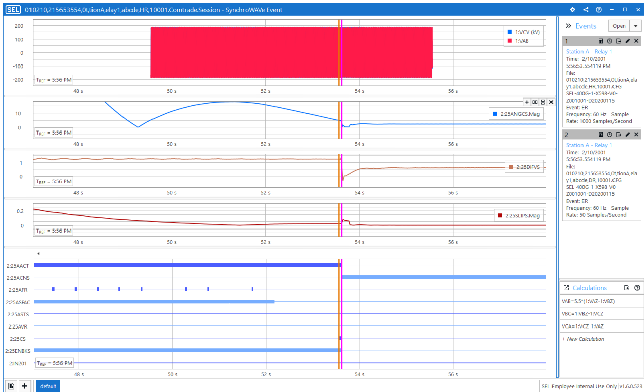
Figure 36 SYNCHROWAVE
