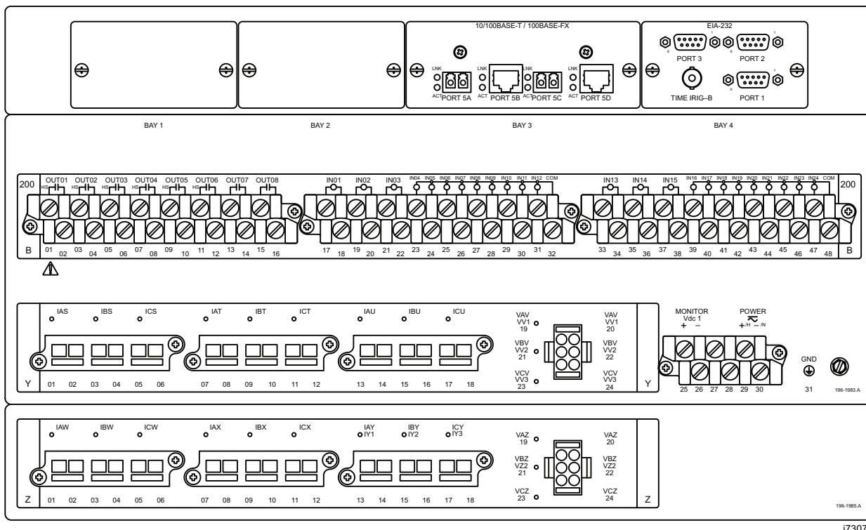
Figure 40 6U Rear-Panel Diagram With Connectorized Terminal Blocks
