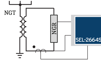
(b) Injecting current via secondary winding of VT when NGR is within neutral of generator
