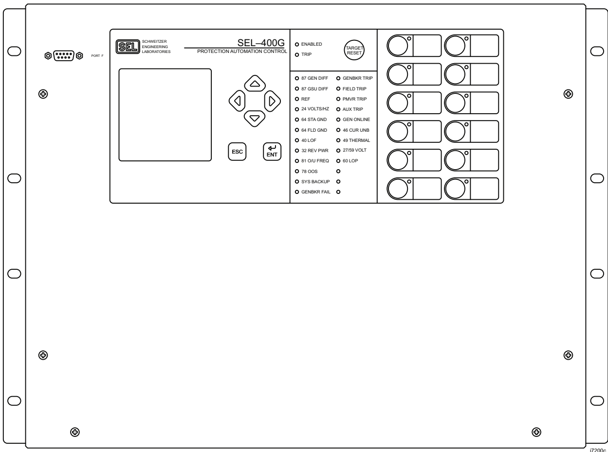
Figure 38 8U Front Panel, Rack-Mount Option
