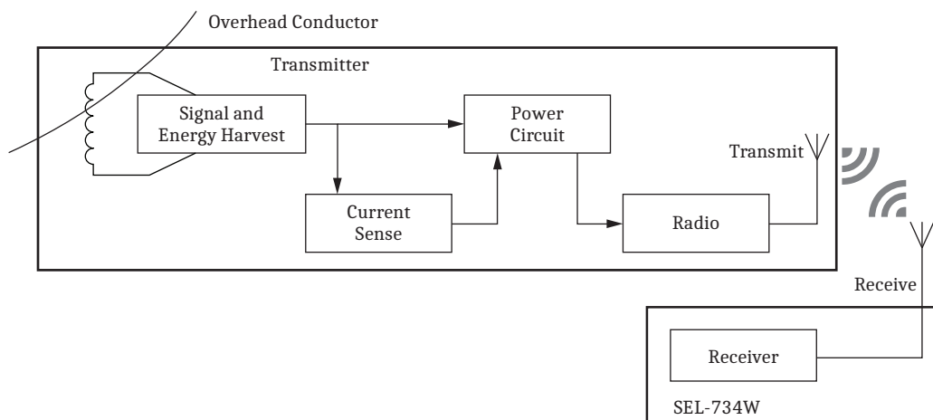
Figure 1 SEL-734W and LINAM WCS Wireless Current Sensor System Overview
