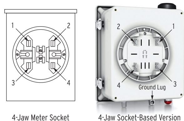
Figure 3 Compact Enclosure Rear Plug and Meter Socket
