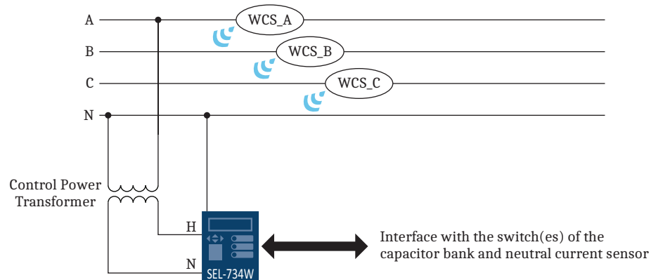
Figure 2 SEL-734W and LINAM WCS System Overview
