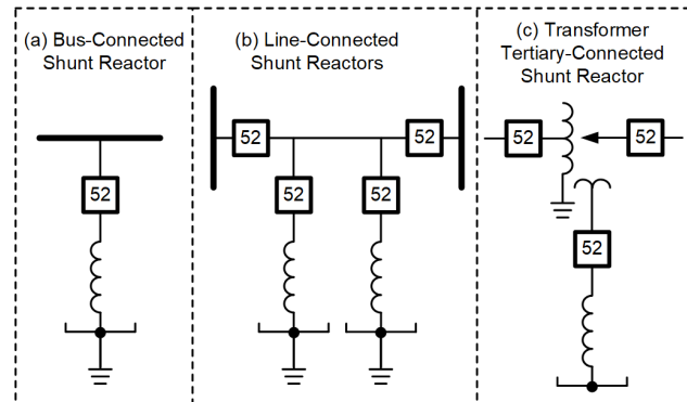
Fig. 1. Types of Shunt Reactors [2]
