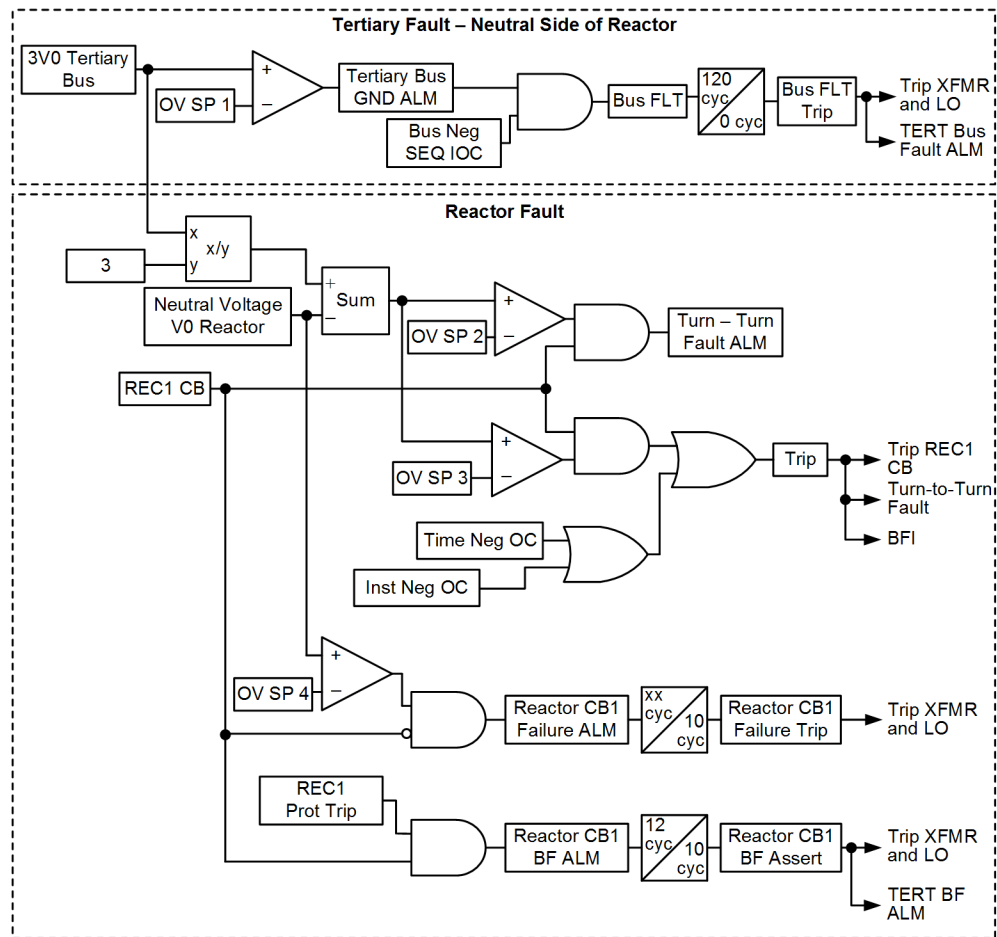
Fig. 7. Tertiary Reactor and Bus Protection Logic Diagram
