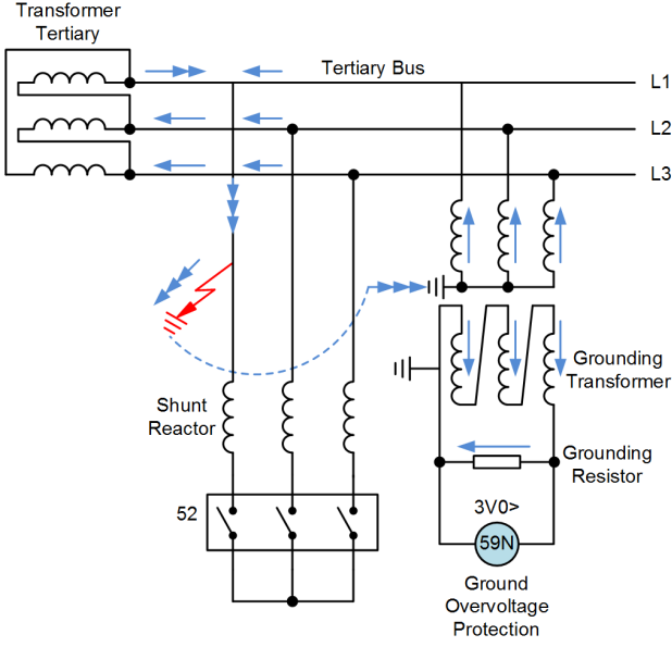
Fig. 4. Dry-Type Shunt Reactor (Ground Overvoltage)
